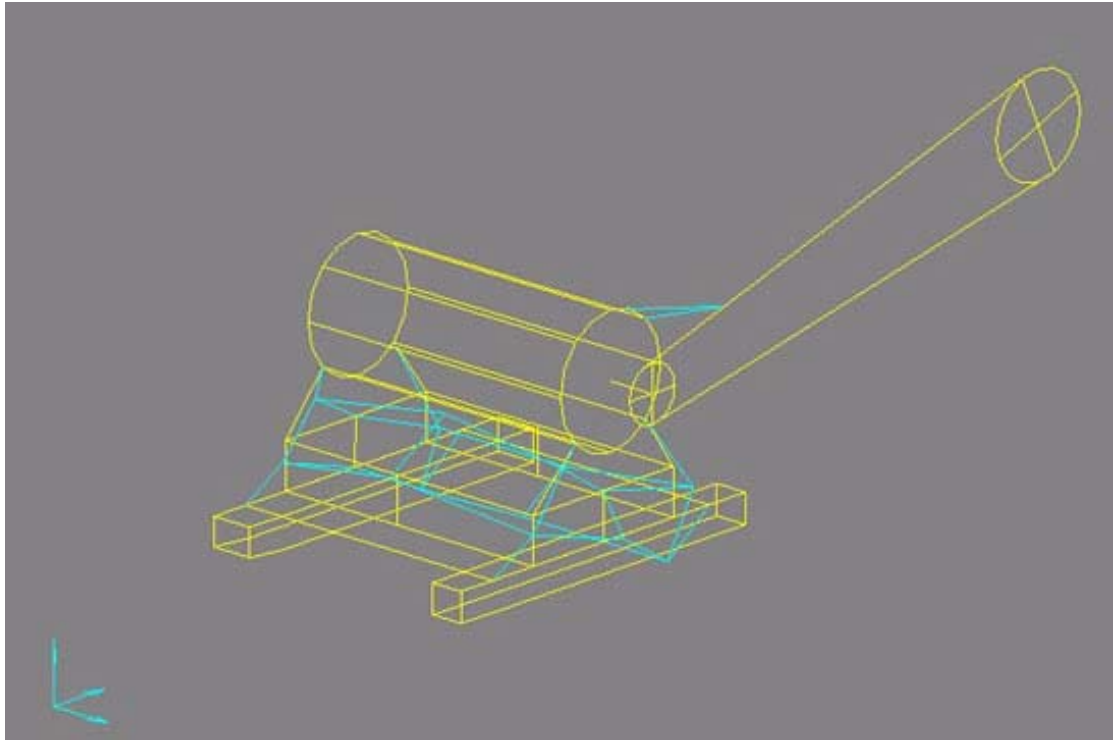
Figure 2: Mode shape of pedestal at 44.6 Hz
