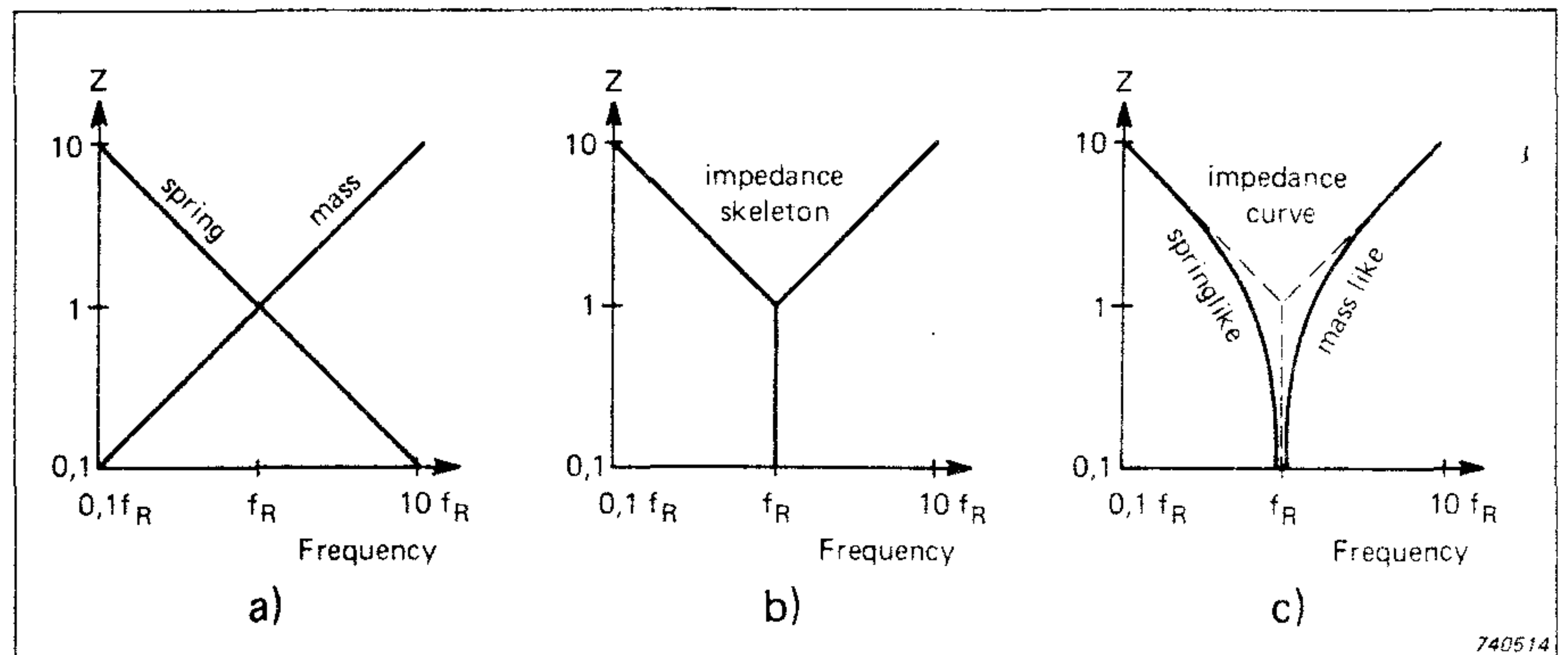
Fig.5. Graphical construction of the mechanical impedance of a mass supported on a spring
