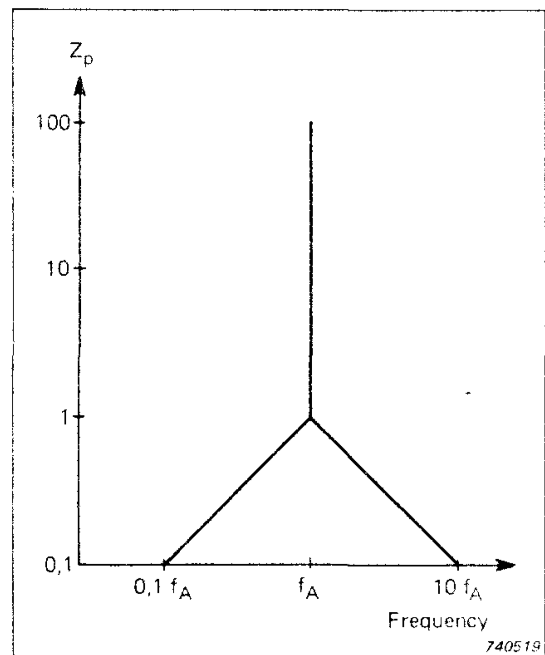
Fig.10. Point impedance skeleton of the sprung mass shown in Fig.6
