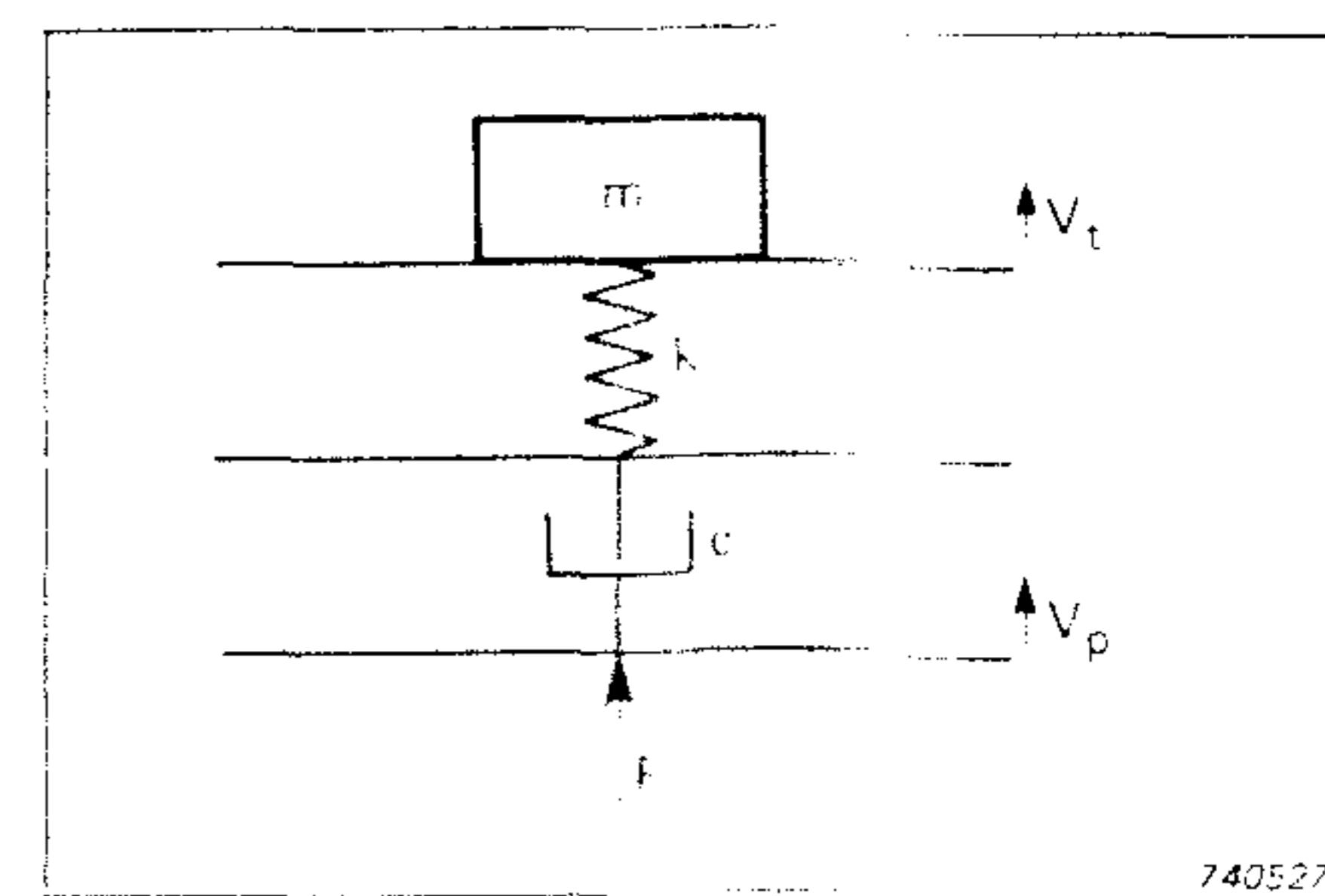
Fig. 18. Damped antiresonant system
