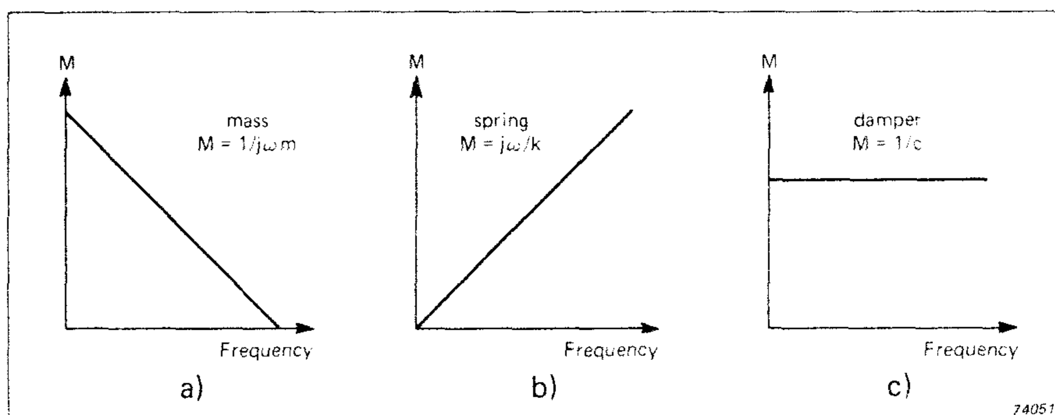
Fig. 3. Mobility for mass, spring and damper
