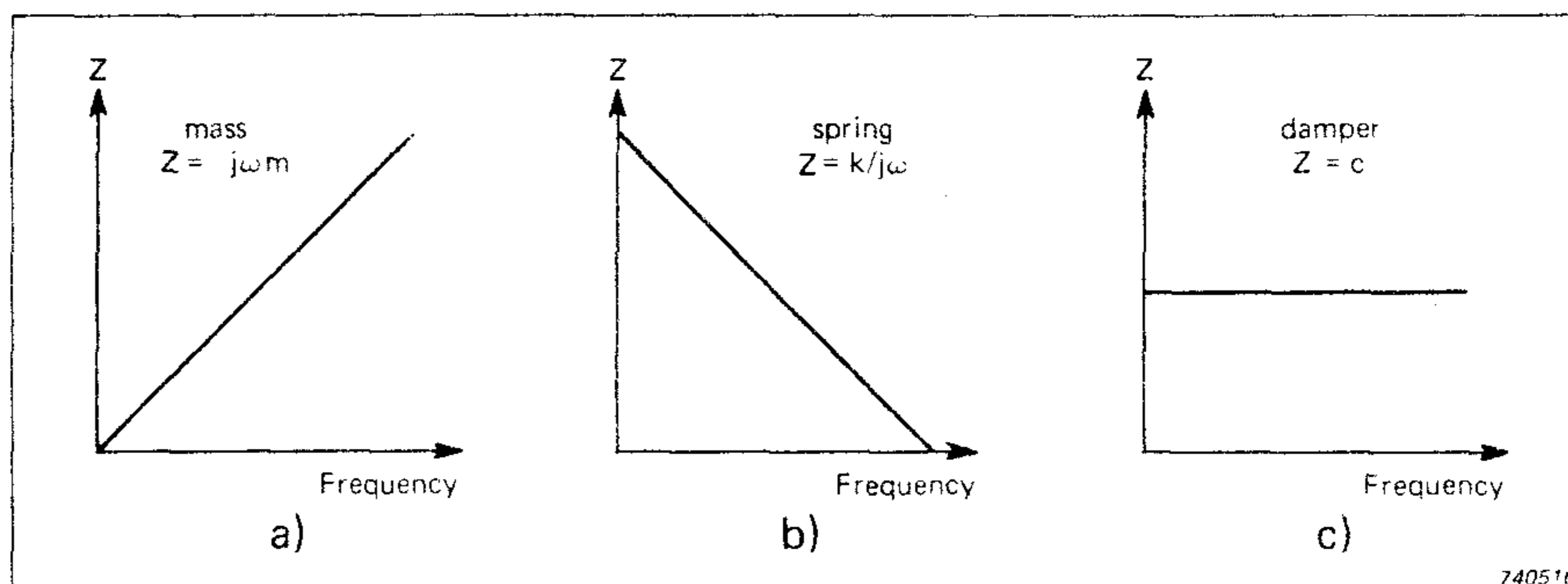
Fig. 2. Mechanical impedance for mass, spring and damper
