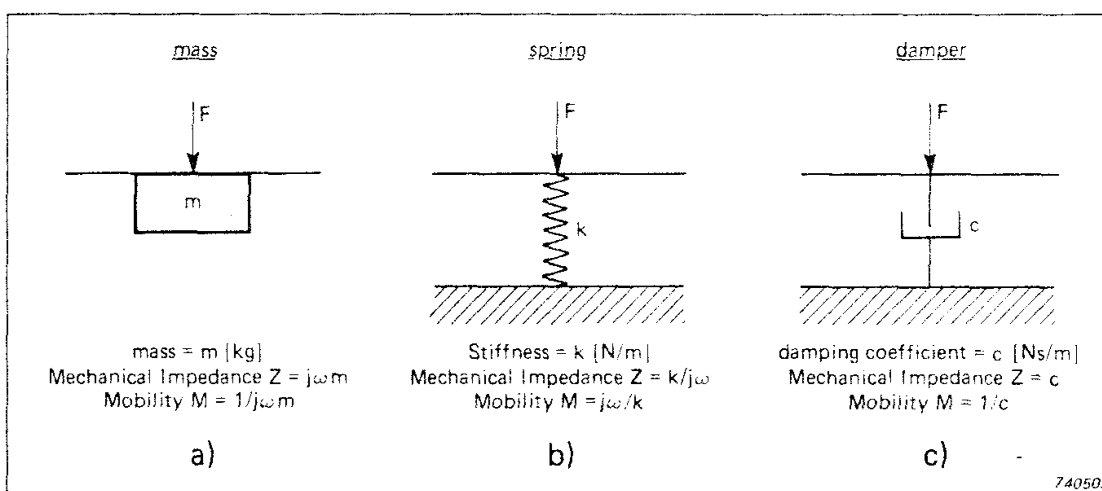
Fig. 1. Signatures for the basic elements
