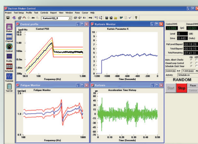
Kurtosis Parameter Control enables better simulation of real world random signals and reduces fatigue test durations
