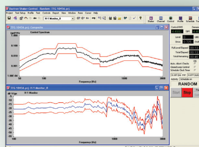
Fatigue Monitoring protects the product and shaker system from damage by using the system inverse transfer function to detect looseness or fatigue and stop the test
