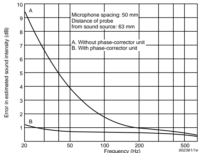
Fig.7 The phase-corrector units fitted to the 4197 suppress vent sensitivity and result in more accurate near-field measurements
