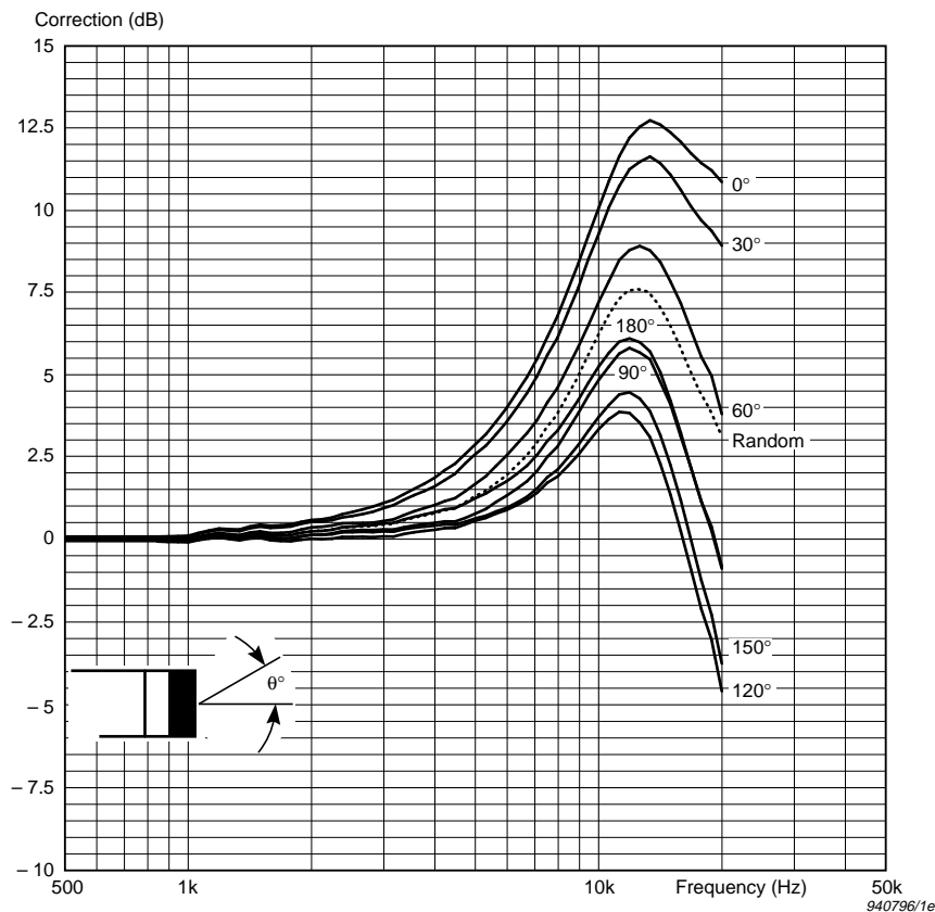
Fig.2.10 Free-field correction curves for the microphone with Random Incidence Corrector DZ 9566
