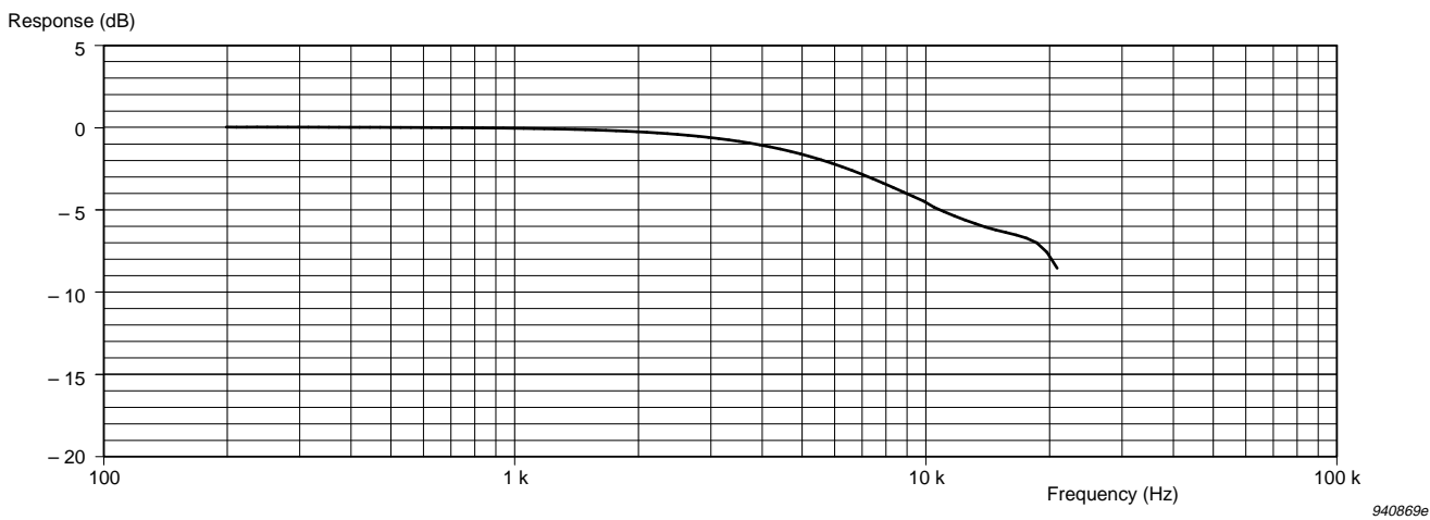
Fig. 3.13 Typical pressure-field response for the microphone
