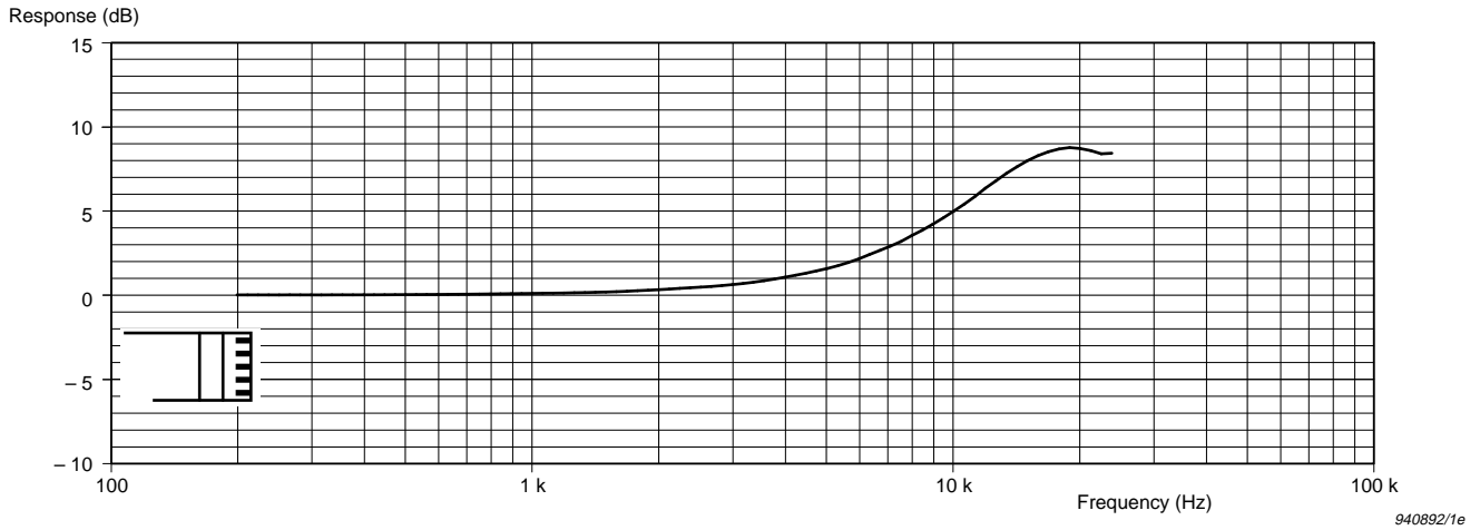
Fig 6.7 Typical free-field response (0° incidence) for the microphone with Protection Grid DB 3421
