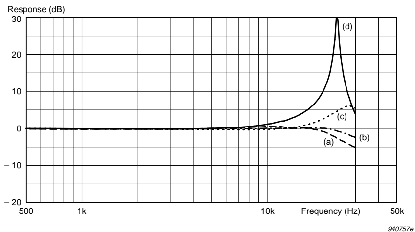
Fig. 7.28 Typical effect of ambient pressure on actuator response (a) at 101.3 kPa (b) -40 kPa change (c) -80 kPa change (d) at 2 kPa
