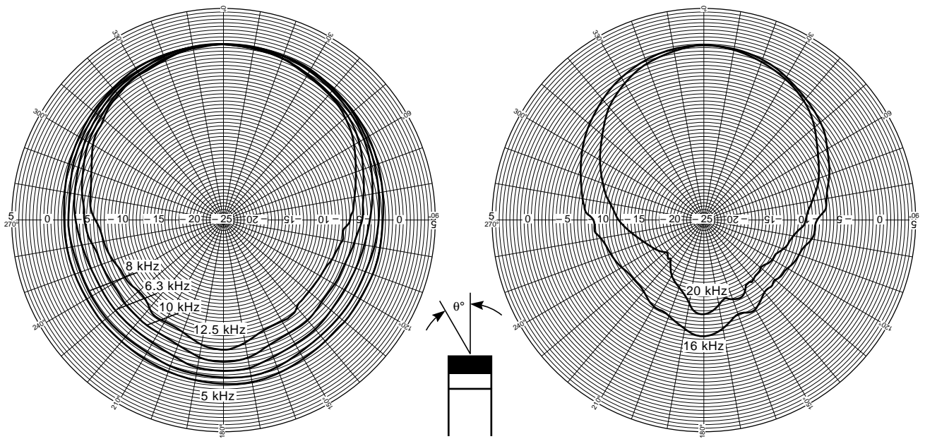
Fig.2.17 Typical directional characteristics of the microphone with Random Incidence Corrector DZ 9566
