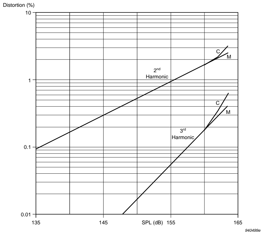
Fig. 5.17 Typical distortion characteristics of the microphone with 1/2" Microphone Preamplifier Type 2669 (C) and unloaded (M)
