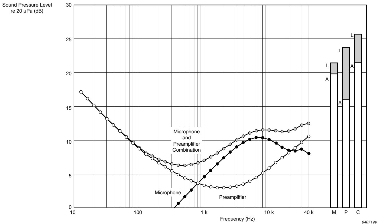
Fig. 5.16 1/3-octave-band inherent noise spectrum. The shaded bar graphs are the broad-band (20Hz to 40kHz) noise levels and the white bar graphs the A-weighted noise levels of the microphone (M), 1/2" Microphone Preamplifier Type 2669 (P) and microphone and preamplifier combination (C)
