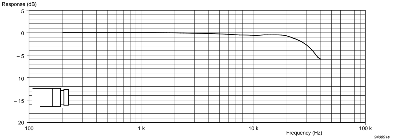
Fig. 5.9 Typical free-field response ( 0^\circ incidence) for the microphone without protection grid
