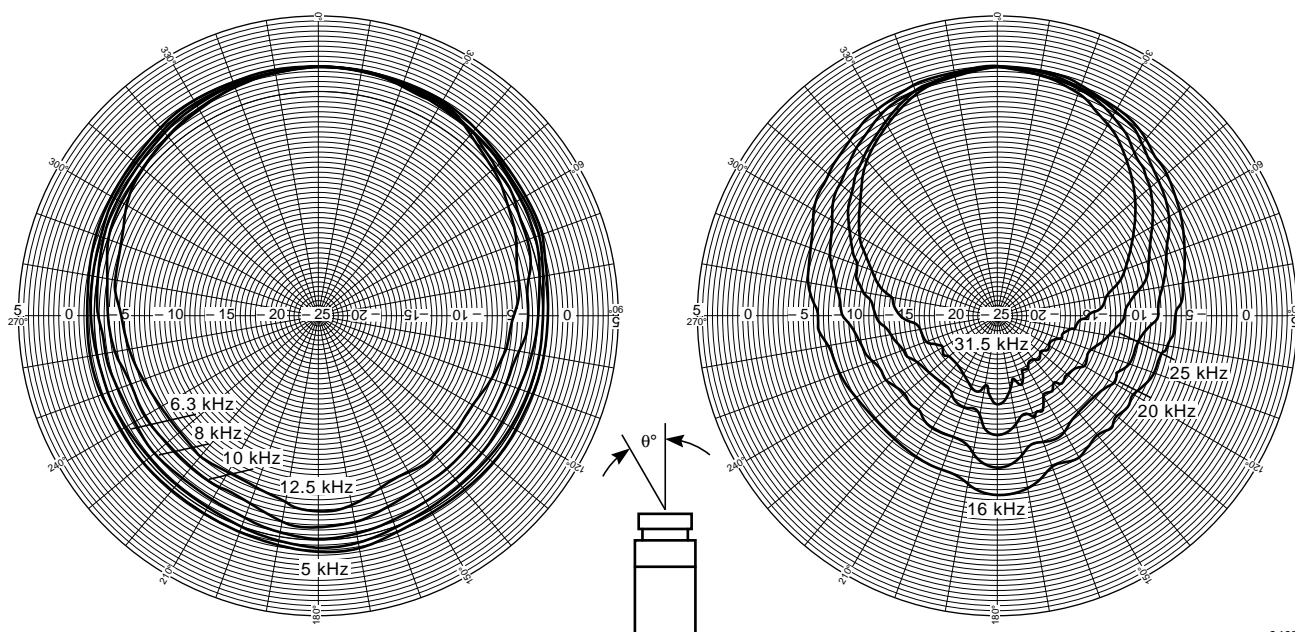
Fig. 3.15 Typical directional characteristics of the microphone without protection grid
