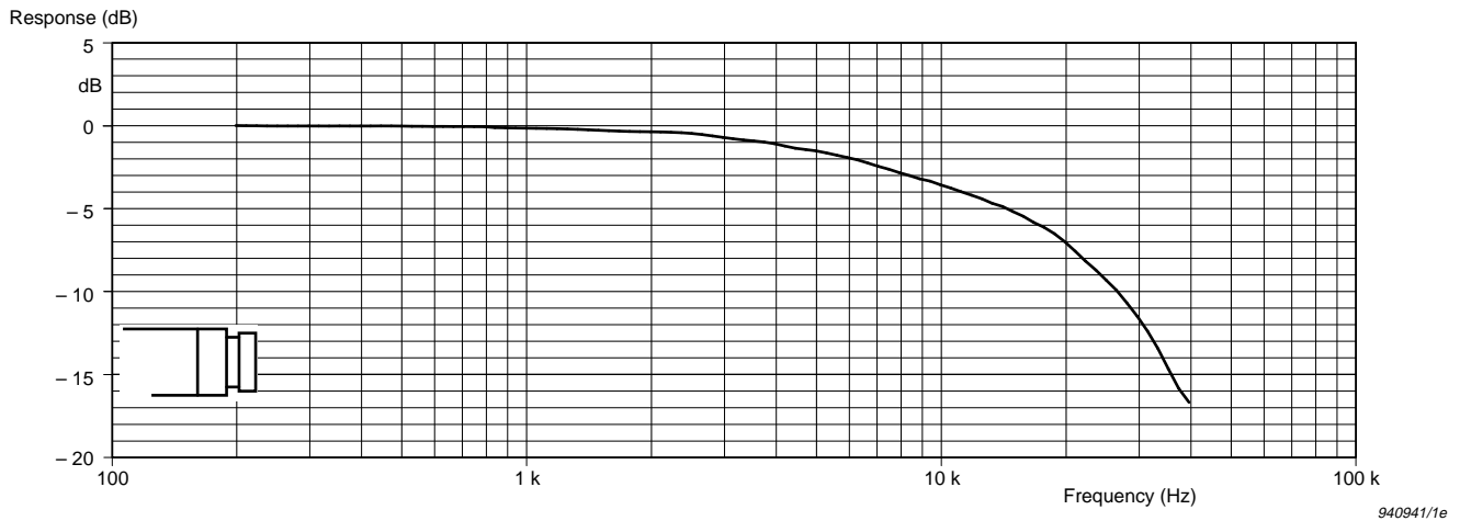
Fig. 5.11 Typical random-incidence response for the microphone without protection grid
