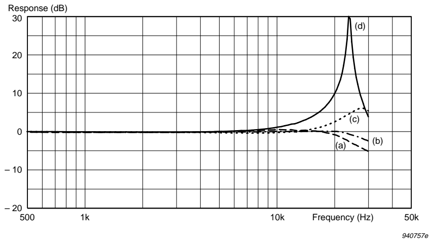
Fig.6.27 Typical effect of ambient pressure on actuator response (a) at 101.3 kPa (b) - 40 kPa change (c) - 80 kPa change (d) at 2 kPa
