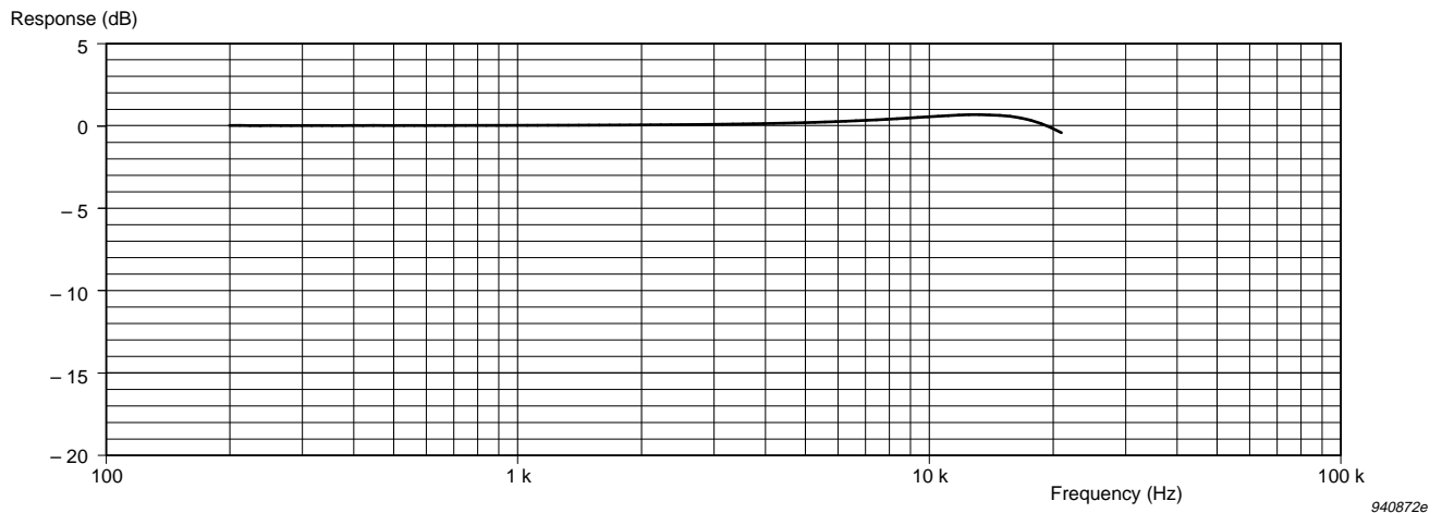
Fig. 7.13 Typical pressure-field response for the microphone
