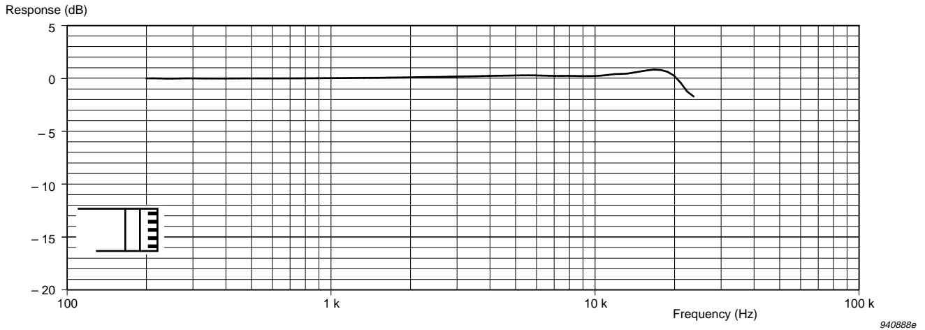
Fig 4.7 Typical free-field response ( 0^\circ incidence) for the microphone with Protection Grid DB 3420
