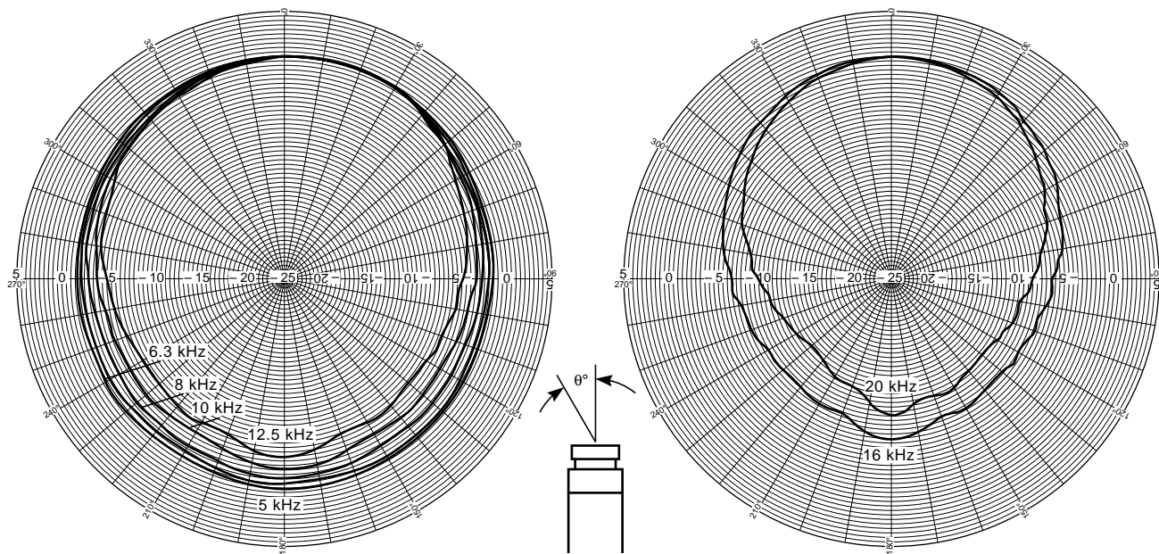
Fig. 2.16 Typical directional characteristics of the microphone without protection grid
