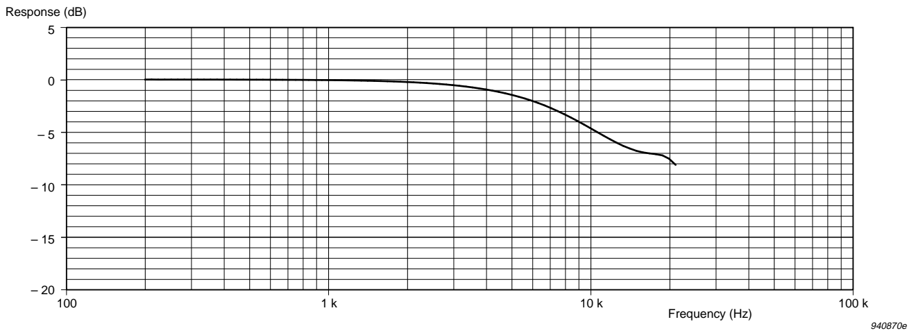
Fig. 4.13 Typical pressure-field response for the microphone
