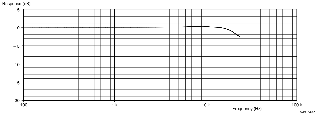
Fig. 7.4 Typical actuator response measured with Electrostatic Actuator UA 0033
