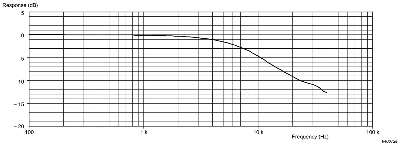
Fig. 5.4 Typical actuator response (magnitude) measured with Electrostatic Actuator UA 0033
