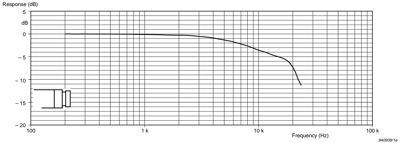
Fig. 4.11 Typical random-incidence response for the microphone without protection grid
