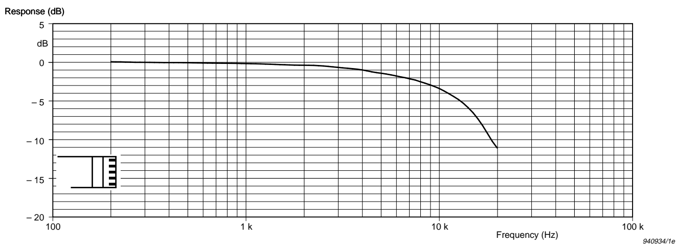
Fig. 2.12 Typical random-incidence response for the microphone with Protection Grid DD 0525
