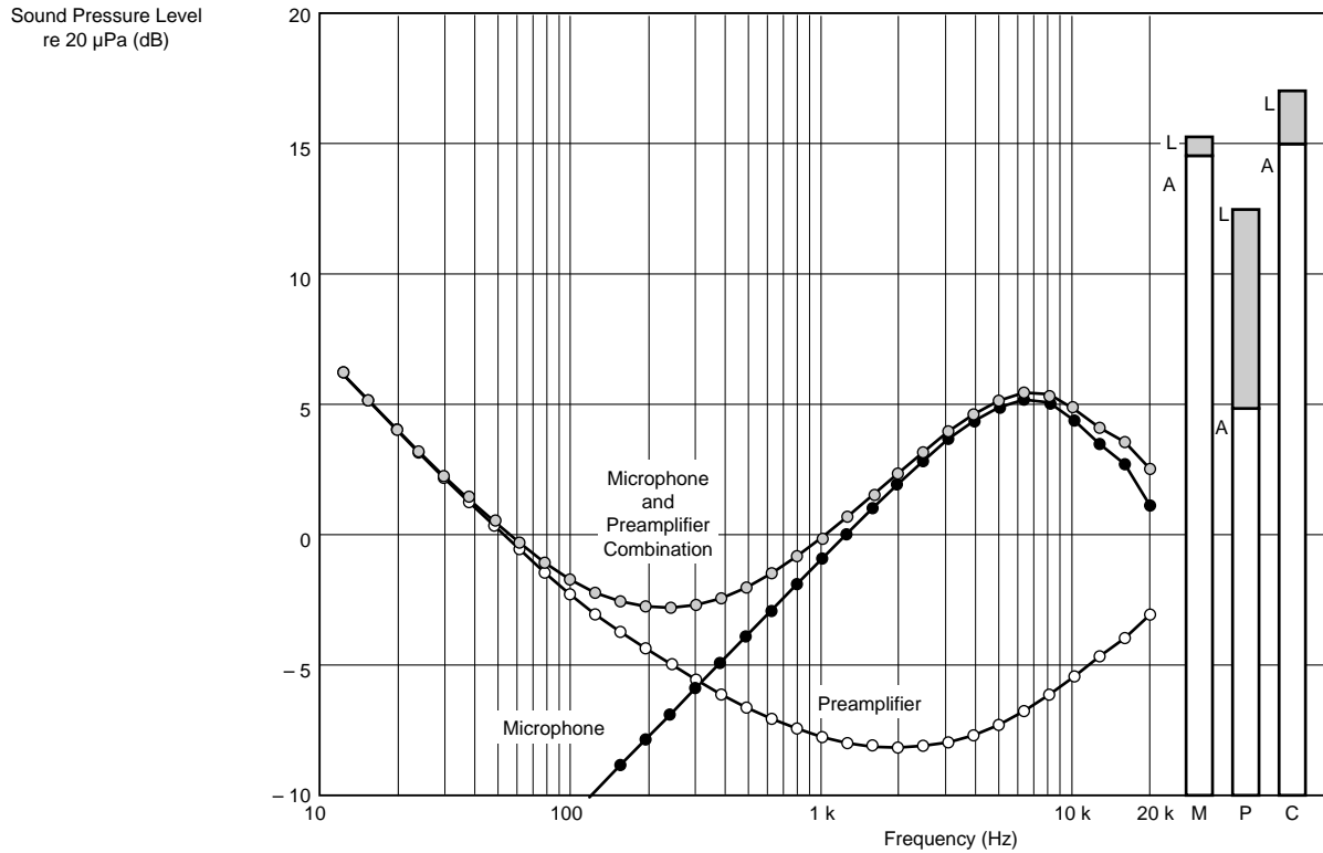
Fig. 4.16 1/3-octave-band inherent noise spectra. The shaded bar graphs are the broad-band (20 Hz to 20 kHz) noise levels and the white bar graphs the A-weighted noise levels of the microphone (M), 1/2" Microphone Preamplifier Type 2669 (P) and microphone and preamplifier combination (C)
