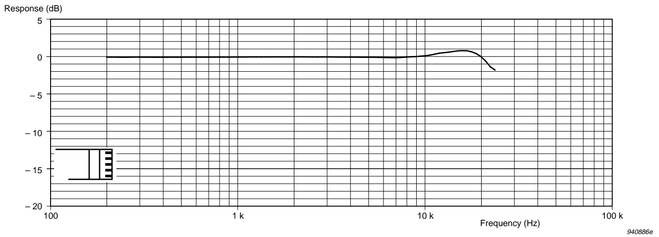
Fig.3.7 Typical free-field response (0° incidence) for the microphone with Protection Grid DB 3420
