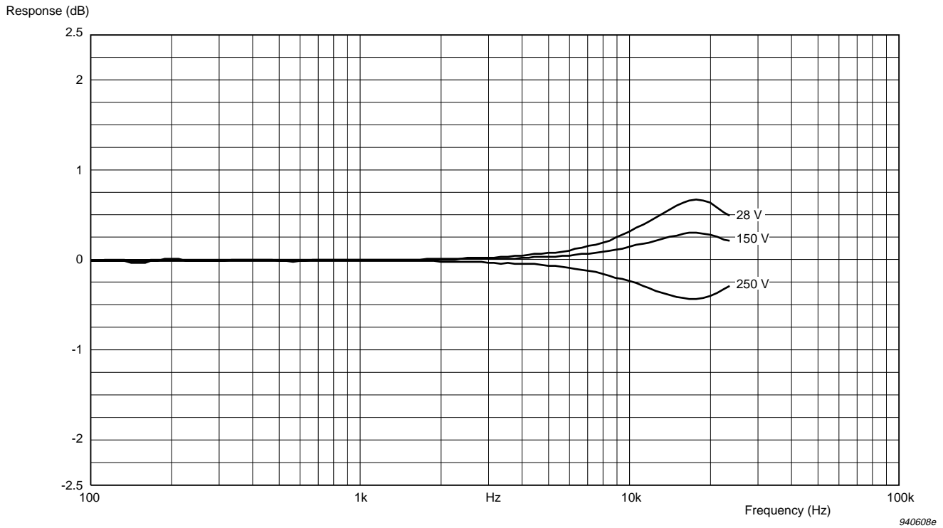
Fig. 7.22 Effect of polarization voltage on frequency response. The curves show the difference from the response with a polarization voltage of 200 V (normalised at 250 Hz)
