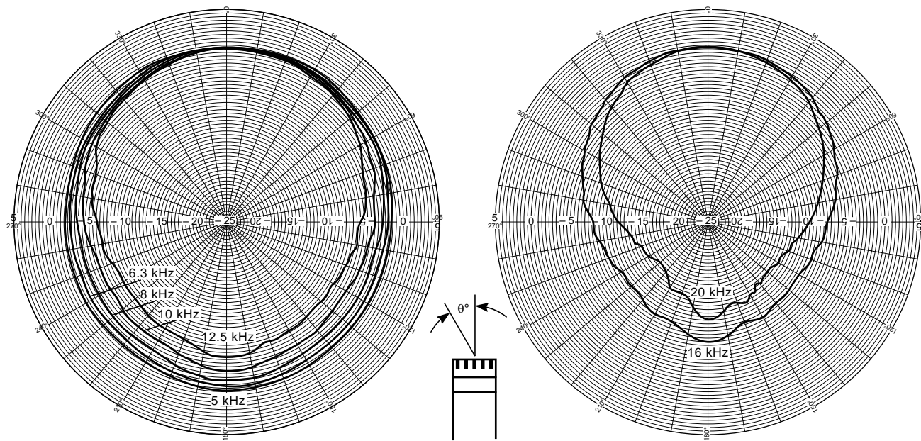
Fig 2.15 Typical directional characteristics of the microphone with Protection Grid DD 0525
