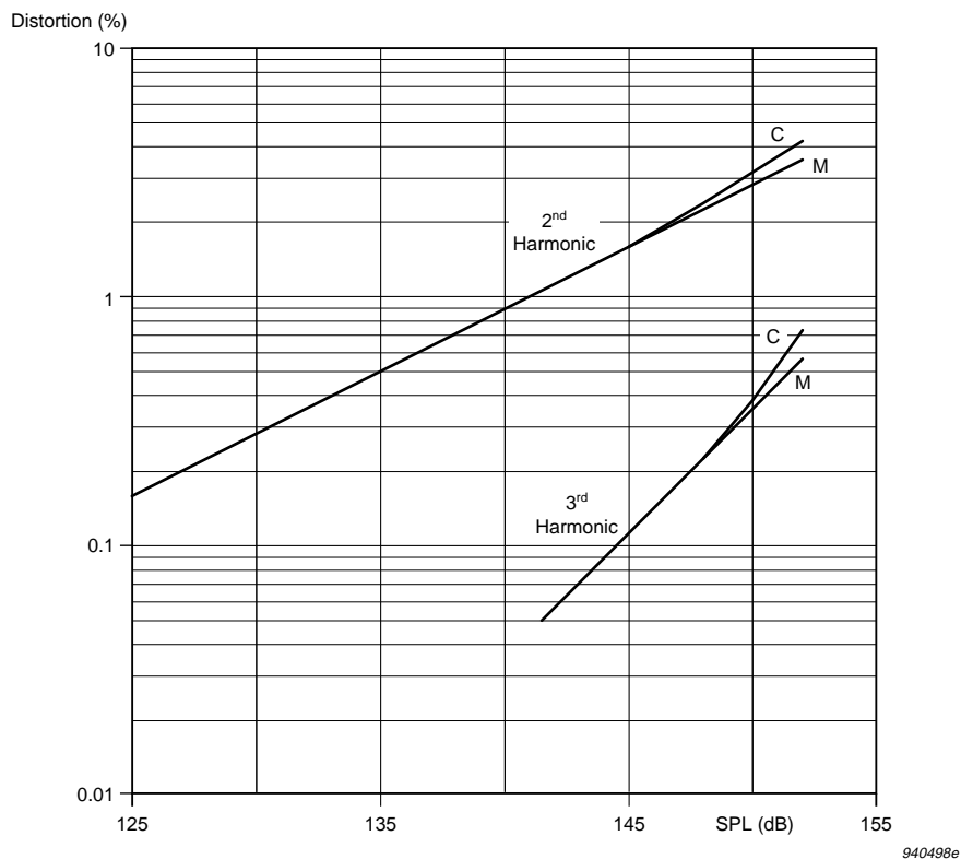
Fig. 4.17 Typical distortion characteristics of the microphone with 1/2" Microphone Preamplifier Type 2669 (C) and unloaded (M)
