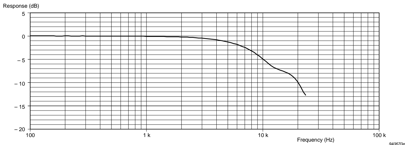
Fig 4.4 Typical actuator response (magnitude) measured with Electrostatic Actuator UA 0033
