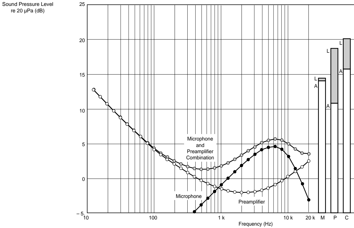
Fig. 2.18 \frac{1}{3} -octave-band inherent noise spectrum. The shaded bar graphs are the broadband (20Hz to 20kHz) noise levels and the white bar graphs the A-weighted noise levels of the microphone (M), \frac{1}{2} " Microphone Preamplifier Type 2669 (P) and microphone and preamplifier combination (C)
