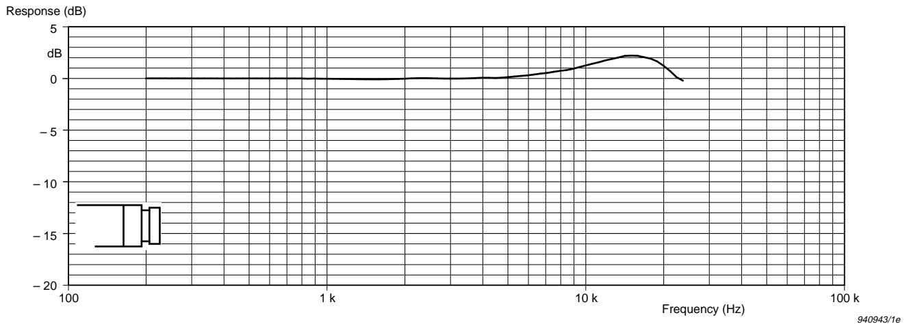
Fig. 6.11 Typical random-incidence response for the microphone without protection grid
