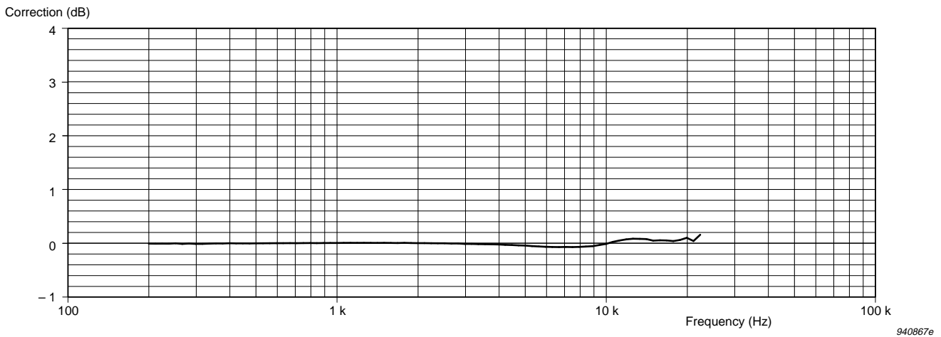
Fig. 5.12 Pressure-field correction for the microphone
