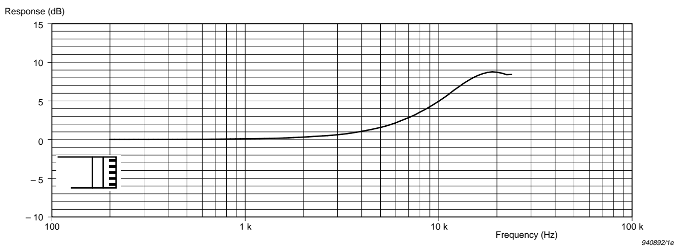
Fig. 7.7 Typical free-field response (0° incidence) for the microphone with Protection Grid DB 3421
