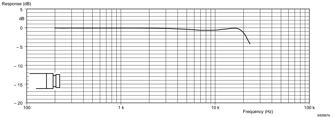
Fig. 3.9 Typical free-field response ( 0^\circ incidence) for the microphone without protection grid
