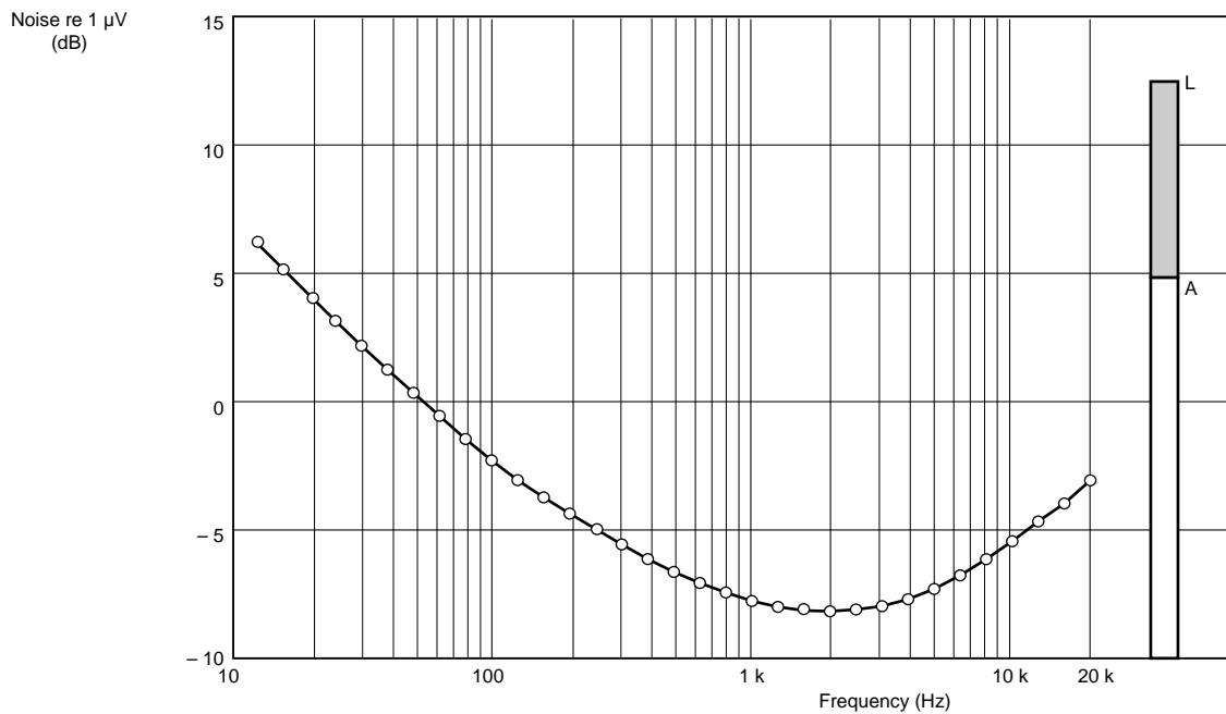
Fig. 8.4 Typical 1/3-octave-band inherent noise spectrum measured with a 15 pF dummy microphone. The shaded bar graph is the broad-band (20 Hz to 20 kHz) noise level and the white bar graph the A-weighted noise level. The circles represent levels at 1/3-octave-band centre frequencies
