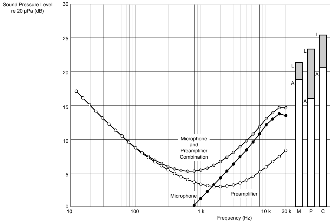
Fig. 6.16 1/3-octave-band inherent noise spectrum. The shaded bar graphs are the broad-band (20Hz to 20kHz) noise levels and the white bar graphs the A-weighted noise levels of the microphone (M), 1/2" Microphone Preamplifier Type 2669 (P) and microphone and preamplifier combination (C)
