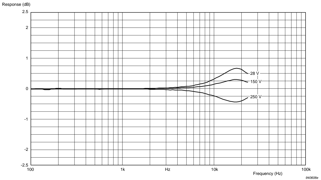
Fig.6.21 Effect of polarization voltage on frequency response. The curves show the difference from the response with a polarization voltage of 200 V (normalised at 250 Hz)
