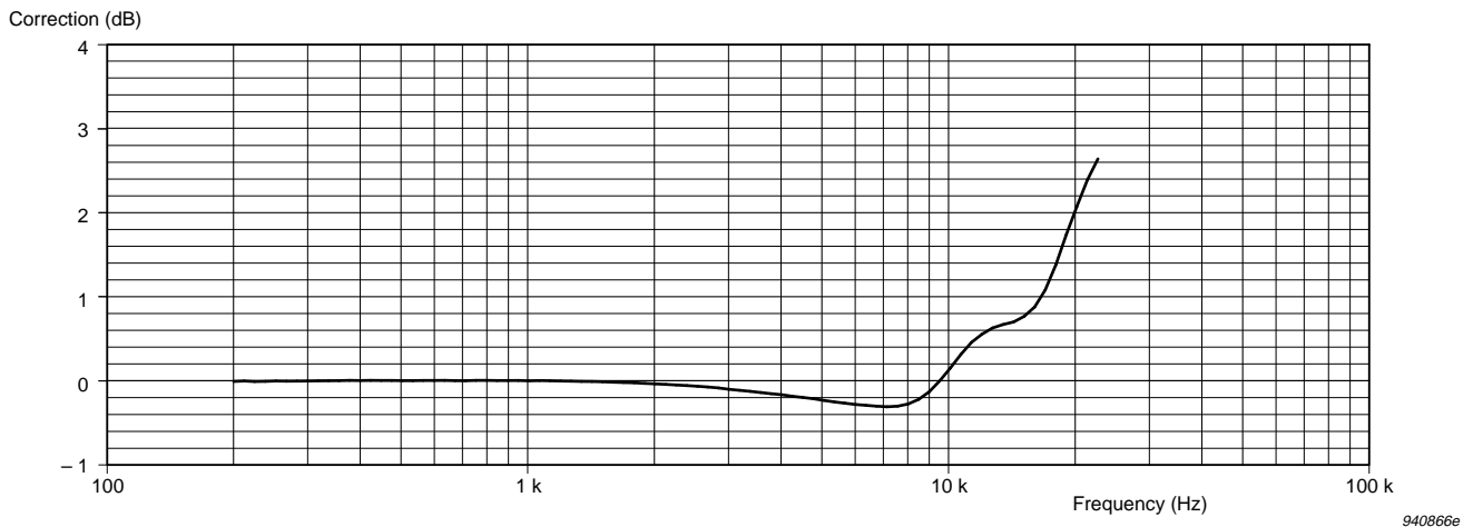
Fig. 4.12 Pressure-field correction for the microphone
