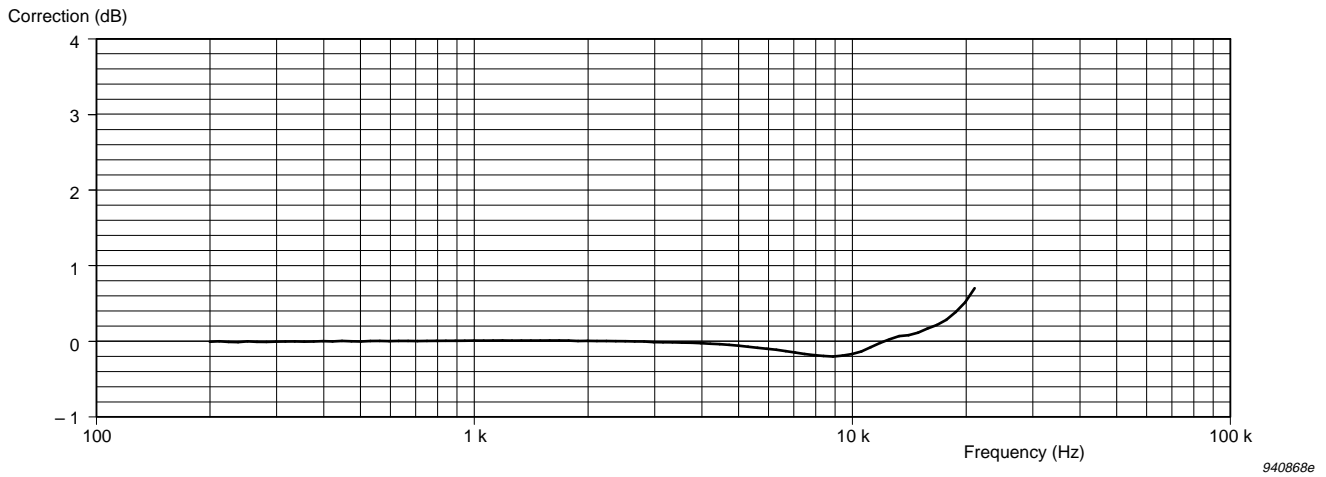
Fig. 6.12 Pressure-field correction for the microphone
