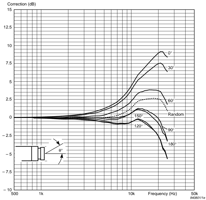
Fig 4.8 Free-field correction curves for the microphone without protection grid
