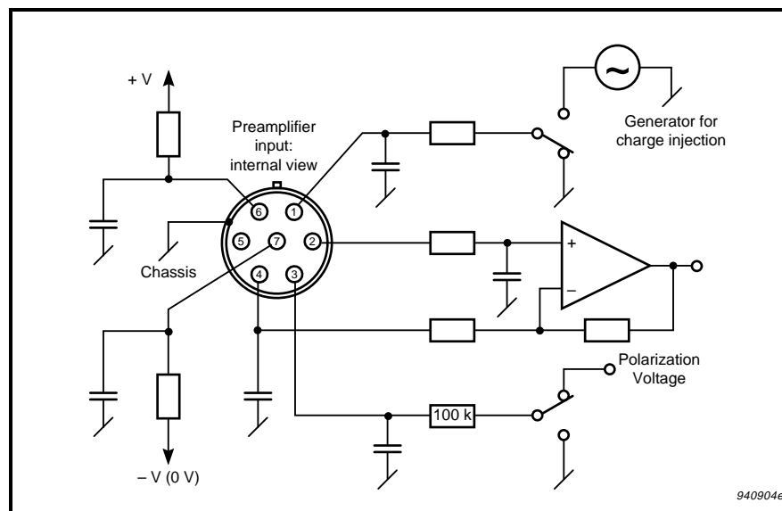
Fig. 8.10 Simplified electronic construction of input circuit of 1/2" Microphone Preamplifier Type 2669 for ensuring compliance with EMC requirements
