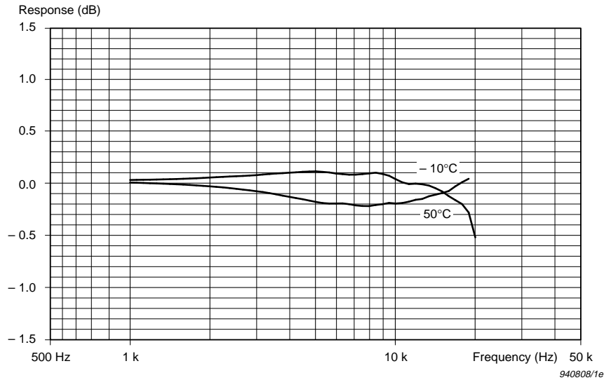
Fig. 4.25 Typical variation in 0°-incidence free-field response (normalized at 250 Hz) as a function of temperature, relative to the response at 20° C (see Fig. 4.7) over the temperature range defined by IEC 651
