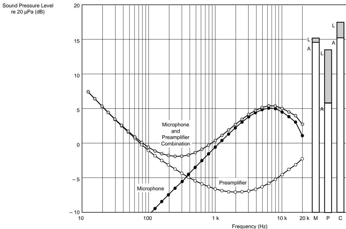
Fig. 3.16 1/3-octave-band inherent noise spectrum. The shaded bar graphs are the broadband (20 Hz to 20 kHz) noise levels and the white bar graphs the A-weighted noise levels of the microphone (M), 1/2" Microphone Preamplifier Type 2669 (P) and microphone and preamplifier combination (C)
