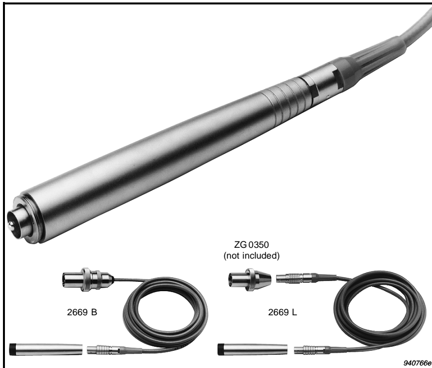
Fig 8.1 \frac{1}{2} " Microphone Preamplifier Type 2669 B and 2669 L shown with LEMO to 7-pin Brüel & Kjær Adaptor ZG 0350 (not included)
