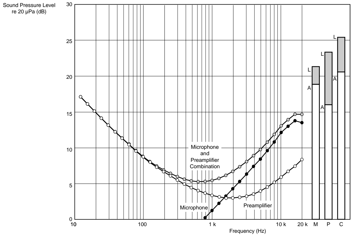
Fig. 7.16 1/3-octave-band inherent noise spectrum. The shaded bar graphs are the broadband (20Hz to 20kHz) noise levels and the white bar graphs the A-weighted noise levels of the microphone (M), 1/2" Microphone Preamplifier Type 2669 (P) and microphone and preamplifier combination (C). Valid for microphone without Adaptor UC 0211
