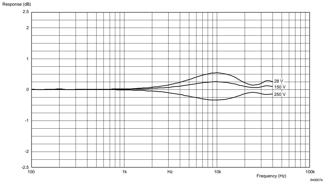
Fig. 5.21 Effect of polarization voltage on frequency response. The curves show the difference from the response with a polarization voltage of 200 V (normalised at 250 Hz)
