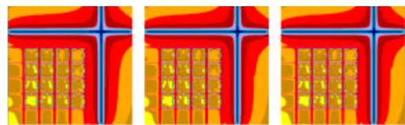
Fig. 10: Calculation of 40401 Receptor Point NoiseLevels on 400 MHz, 52 Road Elements and 96 Buildings (eq. 384 barriers)
