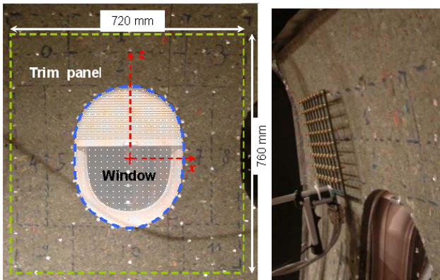
Fig. 9. Window panel. Left : measured area around the left window. Right : DLA during measurement
