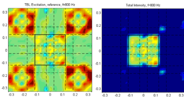
Fig. 5. Intensity maps at 800 Hz directly from FEM model. Left : Reference TBL intensity with no diffuse field. Right : Total intensity with diffuse field.
