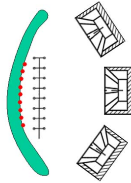
Fig. 3. Cabin panel section with surface calculation points covered by a specific array position. Speakers for measurement of surface properties are shown.
