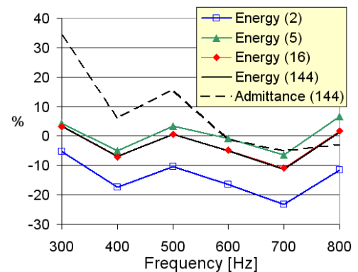
Fig. 7. Sound power error versus number of plane waves used in the simulated measurement of surface properties.
