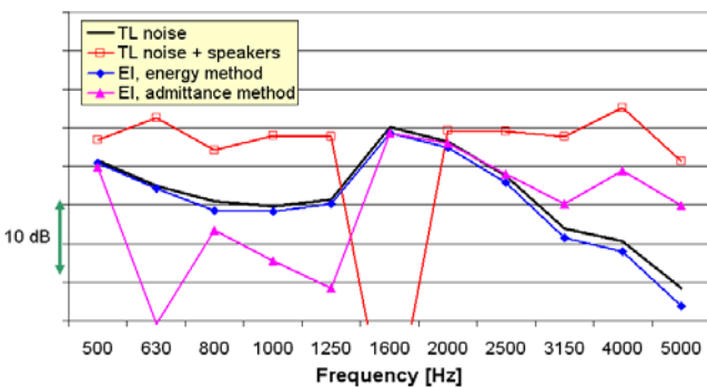
Fig. 14. 1/3-octave sound power spectra for the “window + panel” area defined in relation to Fig. 9, which is the area mapped in Fig. 12 & 13 minus an upper strip.
