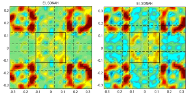
Fig. 6. Entering intensity at 800 Hz.
