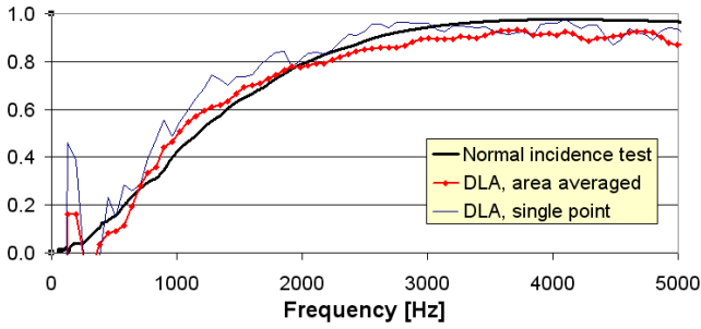
Fig. 11. Absorption coefficient spectra of the panel surface from an impedance tube and from the DLA measurement.
