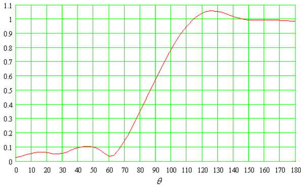
Fig. 2. DLA/SONAH separation of the field component with sources on one side of the array, illustrated through its performance as an angular plane wave filter.
