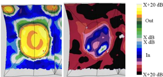
Fig. 12. SONAH total intensity maps.
