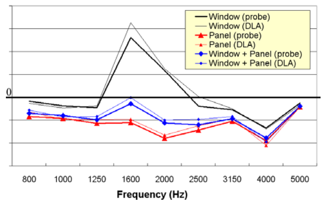
Fig. 10. Area averaged total intensity 1/3-octave spectra. The y-axis shows linear intensity ( W/m^2 ).
