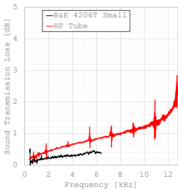
(10a) Sound Transmission Losses
