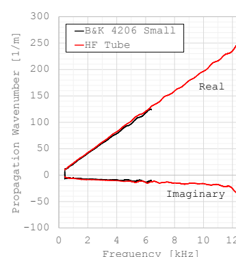
(12c) Propagation Wavenumbers
