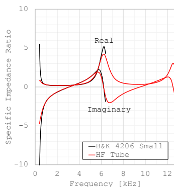
(9b) Specific Impedance Ratios
