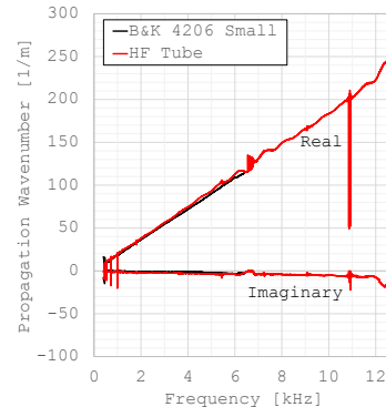
(10c) Propagation Wavenumbers
