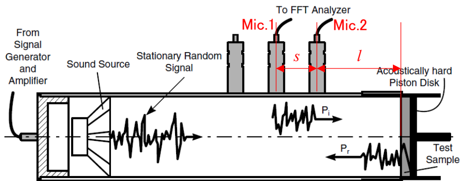
Figure 1 – Setup for the Impedance tube for SAC measurement
