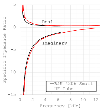
(8b) Specific Impedance Ratios
