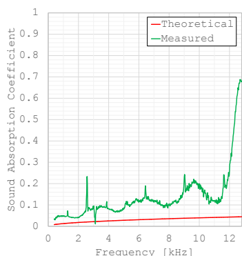
(7b) 25 mm Air
