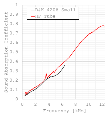
(8c) Sound Absorption Coefficients
