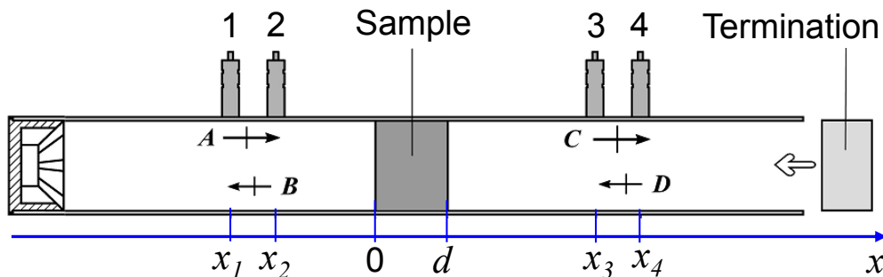
Figure 2 – Setup for the Impedance tube for STL measurement
