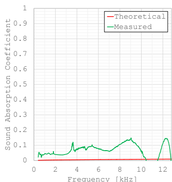
(7a) 5 mm Air
