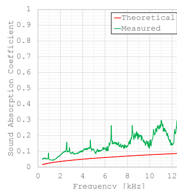
(7c) 50 mm Air
