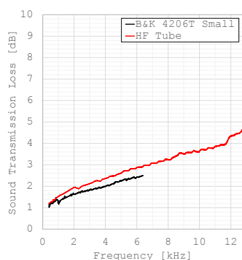
(12a) Sound Transmission Losses
