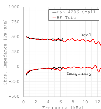
(12b) Characteristic Impedances
