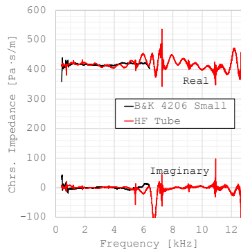
(10b) Characteristic Impedances
