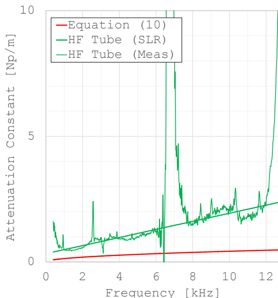
Figures 6 – Comparison of the theoretical and measured attenuation coefficient of 25 mm thickness air cavities. SLR is a linear regression of the measured data
