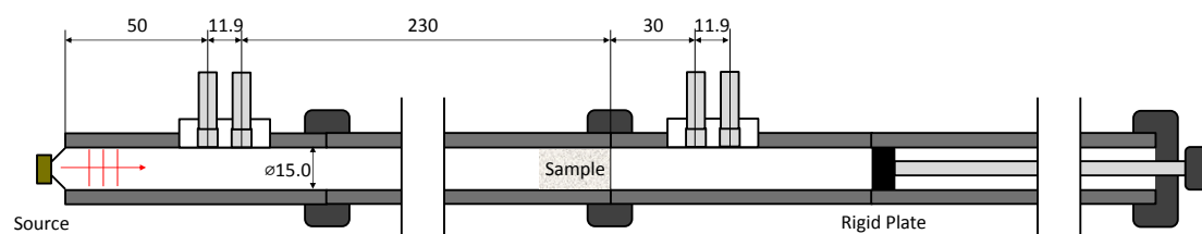
(4a) Outline drawing (hard wall termination)
