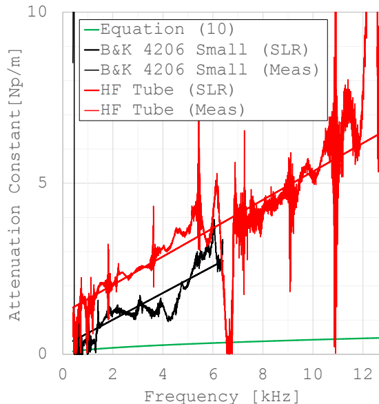
Figure 11 – Comparison of the theoretical and measured attenuation coefficient of 25 mm thickness air cavity. SLR is a linear regression of the measured data
