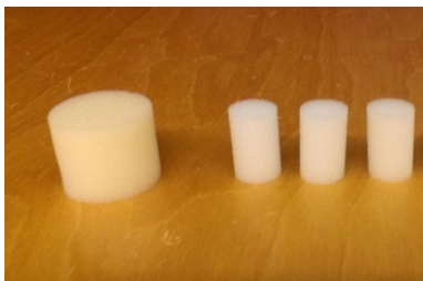
(9a) Image of samples (Left: for Brüel & Kjær 4206 small tube, Right: for HF tube)
