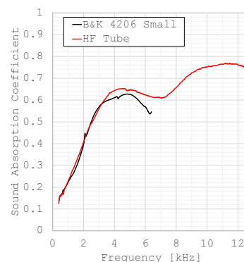
(9c) Sound Absorption Coefficients
