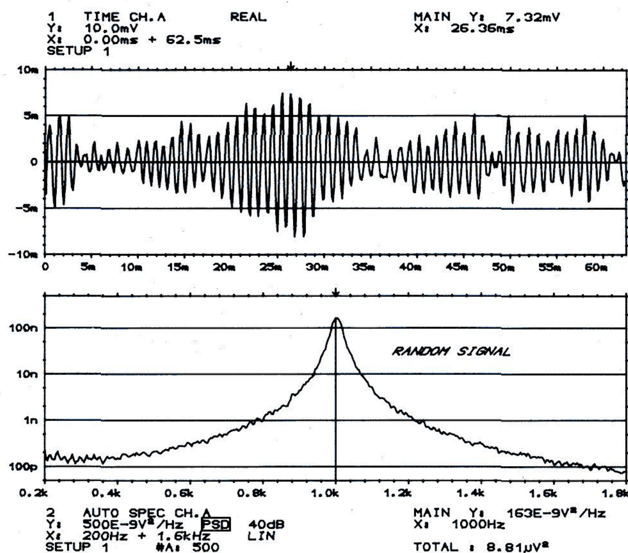
Fig. 1. Time record and frequency spectrum for a stationary, random process. The frequency spectrum is scaled as the power spectral density.
