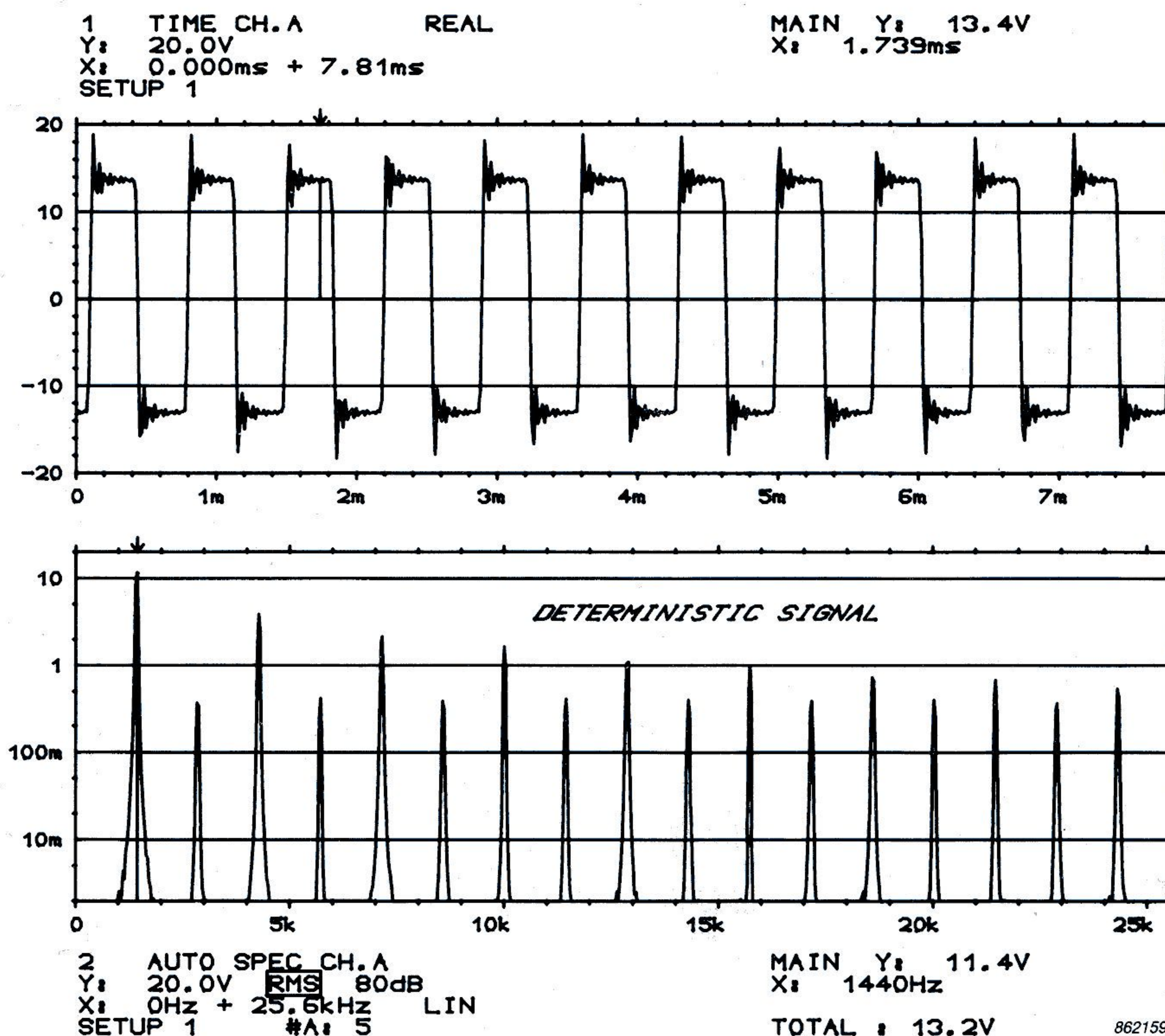
Time record and frequency spectrum for a stationary, deterministic signal. The frequency spectrum is scaled as the root mean square of the signal.
