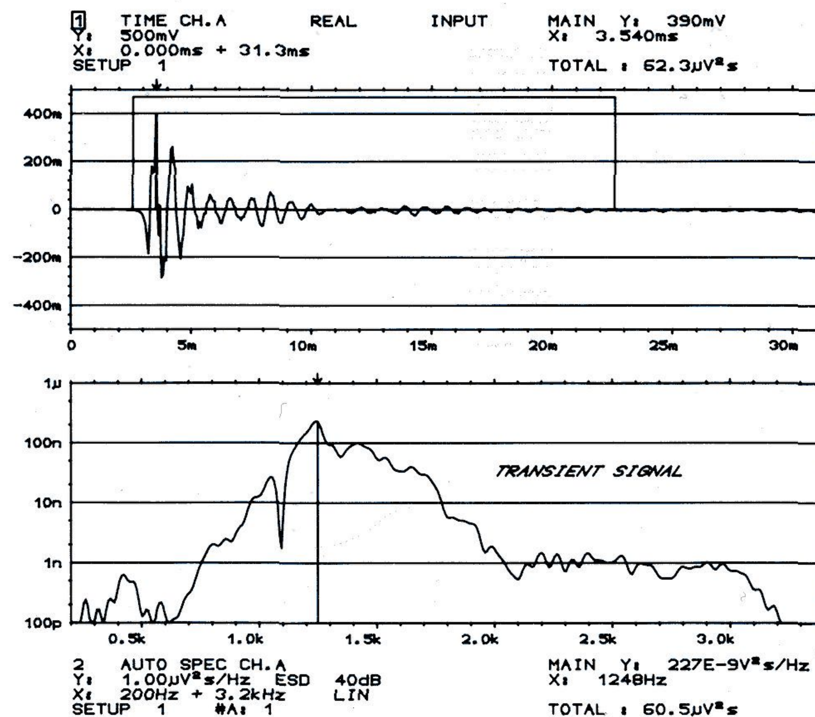
Fig. 2. Time record and frequency spectrum for a transient signal. A transient time-weighting function is used in the analysis of the time record, and the frequency spectrum is scaled as the energy spectral density.
