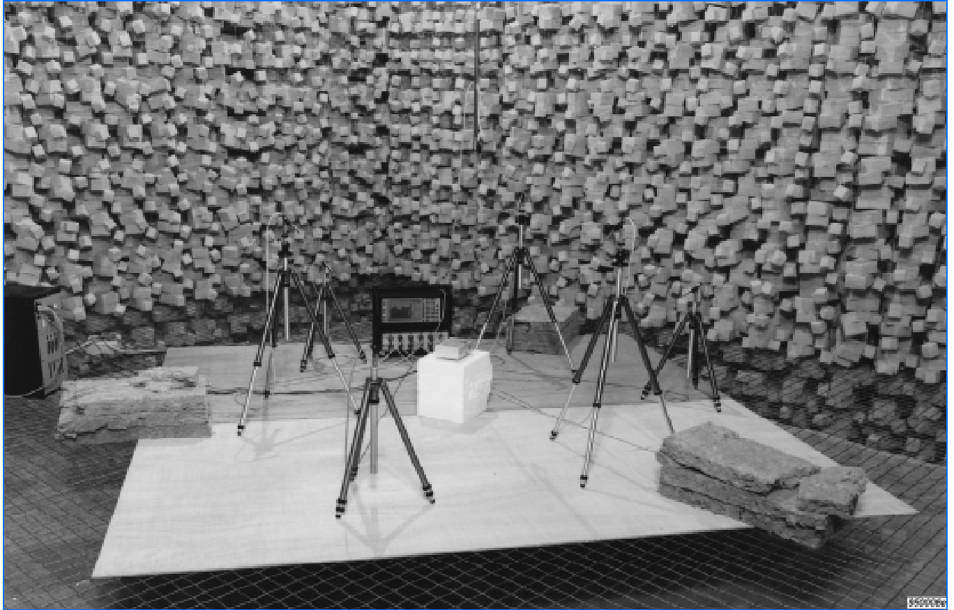
Fig.1 Measuring a tape streamer according to ISO 3745 in the anechoic room. According to ISO 7779, the tape streamer must be placed 25 cm above the reflecting floor. 10 microphones are placed on a hemisphere. Multiplexer and analyzer can be seen behind the tape streamer, the PC is located outside the room
