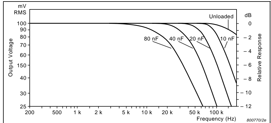
Fig. 2 Typical small signal high frequency response of Type 2634 for different capacity loads at the output. Assuming a cable capacitance of 100 pF/m, a 10 nF load is equivalent to 100 m of cable at the output
