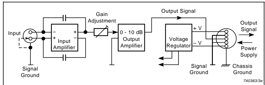
Fig. 1 Simplified block diagram of the Charge Amplifier Type 2634
