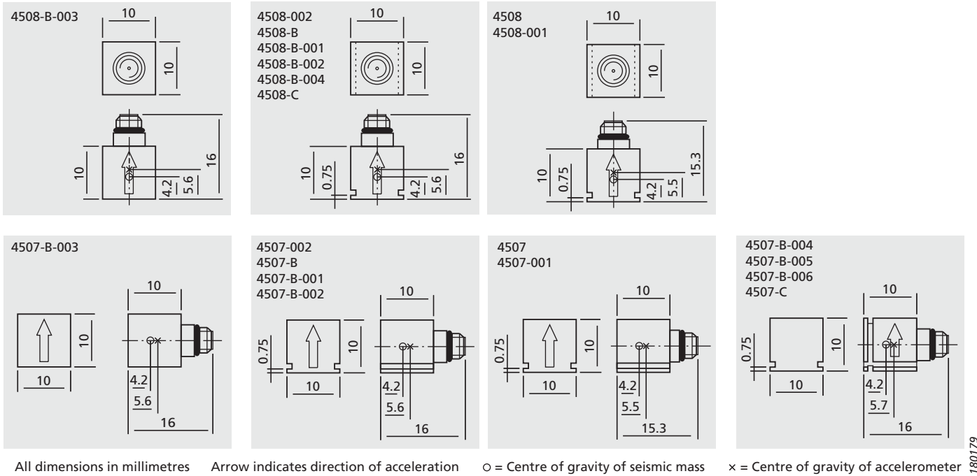
Fig. 10 Dimensions of the variants, grouped by dimensions and arranged by family ( top : Type 4508 family, bottom : Type 4507 family) and mounting slots ( left : no mounting slots, middle : one pair of mounting slots, right : three pairs of mounting slots)
