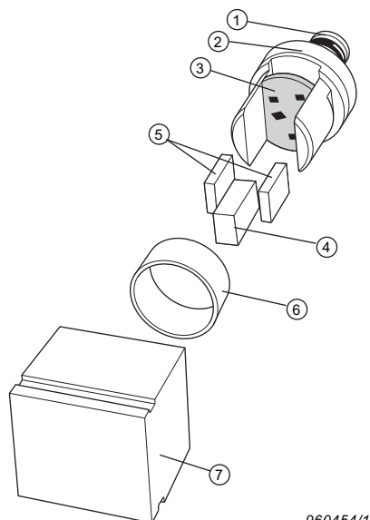
Fig. 2 Exploded view of Type 4508 showing the ThetaShear design and built-in CCLD preamplifier: (1) 10–32 UNF connector (2) Top (3) Preamplifier (4) Piezoelectric plates (5) Seismic mass (6) Clamping ring (7) Titanium housing
