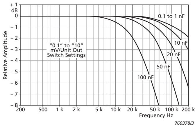
Fig. 8 Influence of the input load capacitance on the high-frequency response of a Brüel & Kjær charge amplifier
