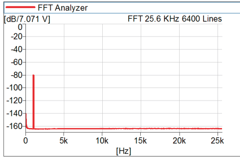
Fig. 5 160 dB analysis in one range. An FFT measuring a 1 kHz signal 80 dB below full scale ( 7 V_{rms} ). Note that noise and all spurious components measure 160 dB below full-scale input
