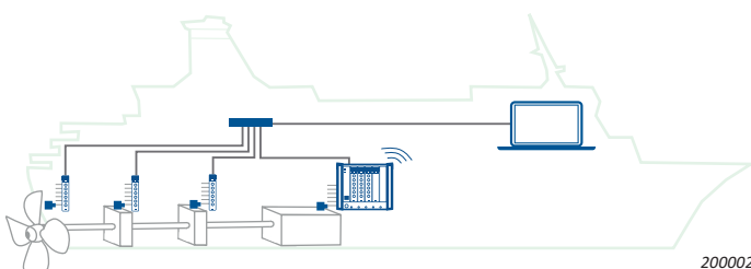
Fig. 1 PTP enables distributed systems where modules are situated close to the measurement object. Using a LAN cable for data transfer, PoE and PTP drastically reduces cabling
