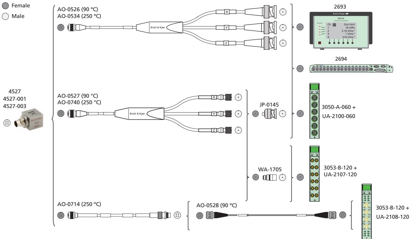
Fig. 3 Typical configurations with Types 4527, 4527-001 and 4527-003
