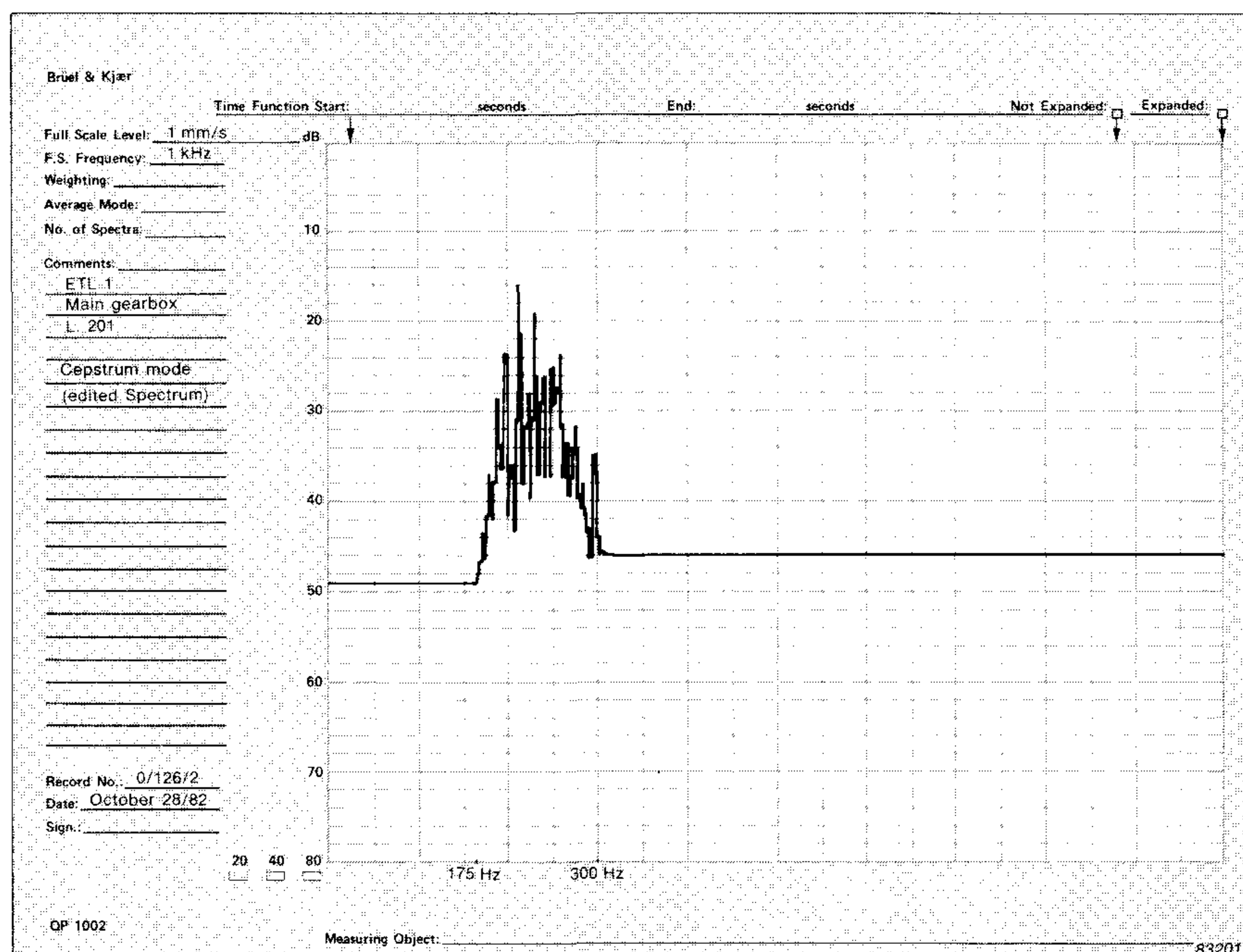
Fig. 9. "Edited" spectrum before the calculation of cepstrum, so as to eliminate harmonics far from the meshing frequency
