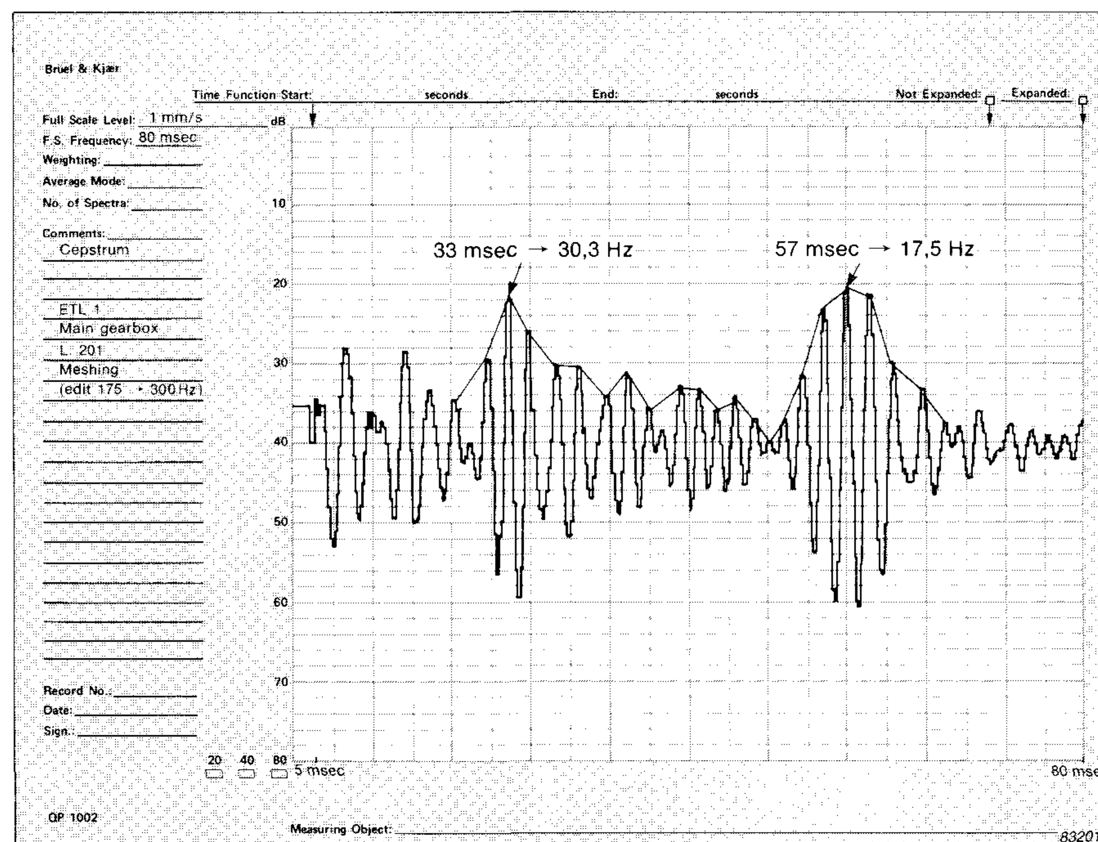
Fig. 10. Cepstrum calculated from Fig. 9. The two lines at 33 msec. and 57 msec. correspond to the rotation speeds of the pinions
