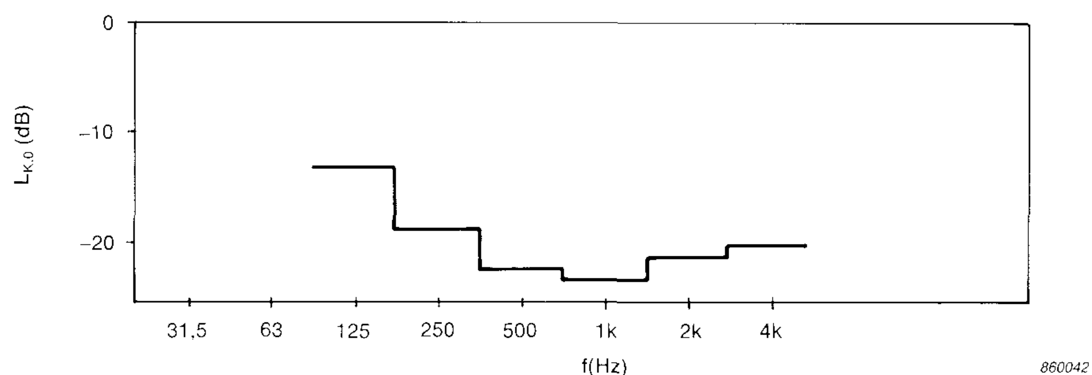
Fig. 10. The measured Residual Intensity Index for the 4433/Probe for a microphone spacing of 12 mm
