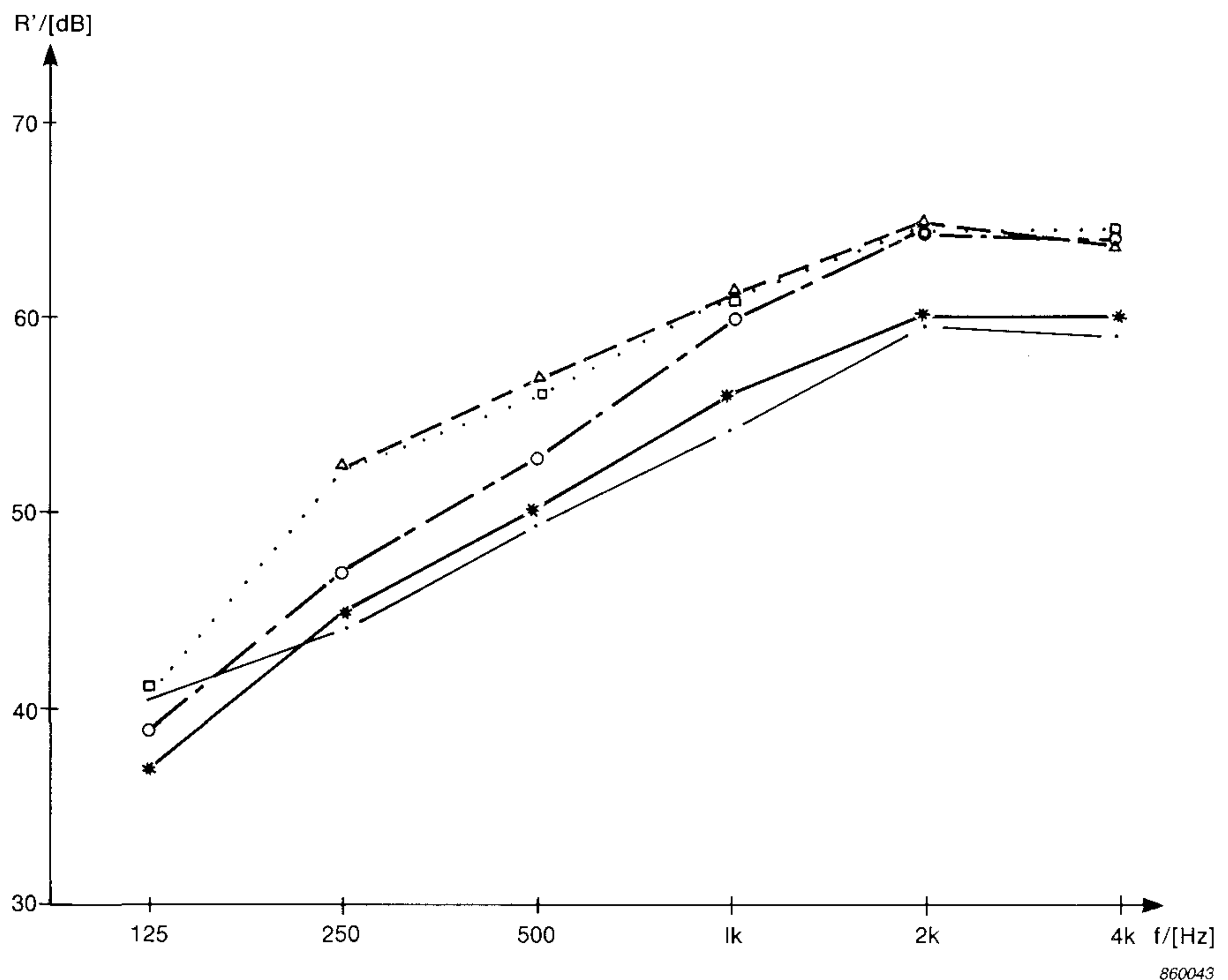
Fig. 7. Measurements of apparent sound reduction index R' .
