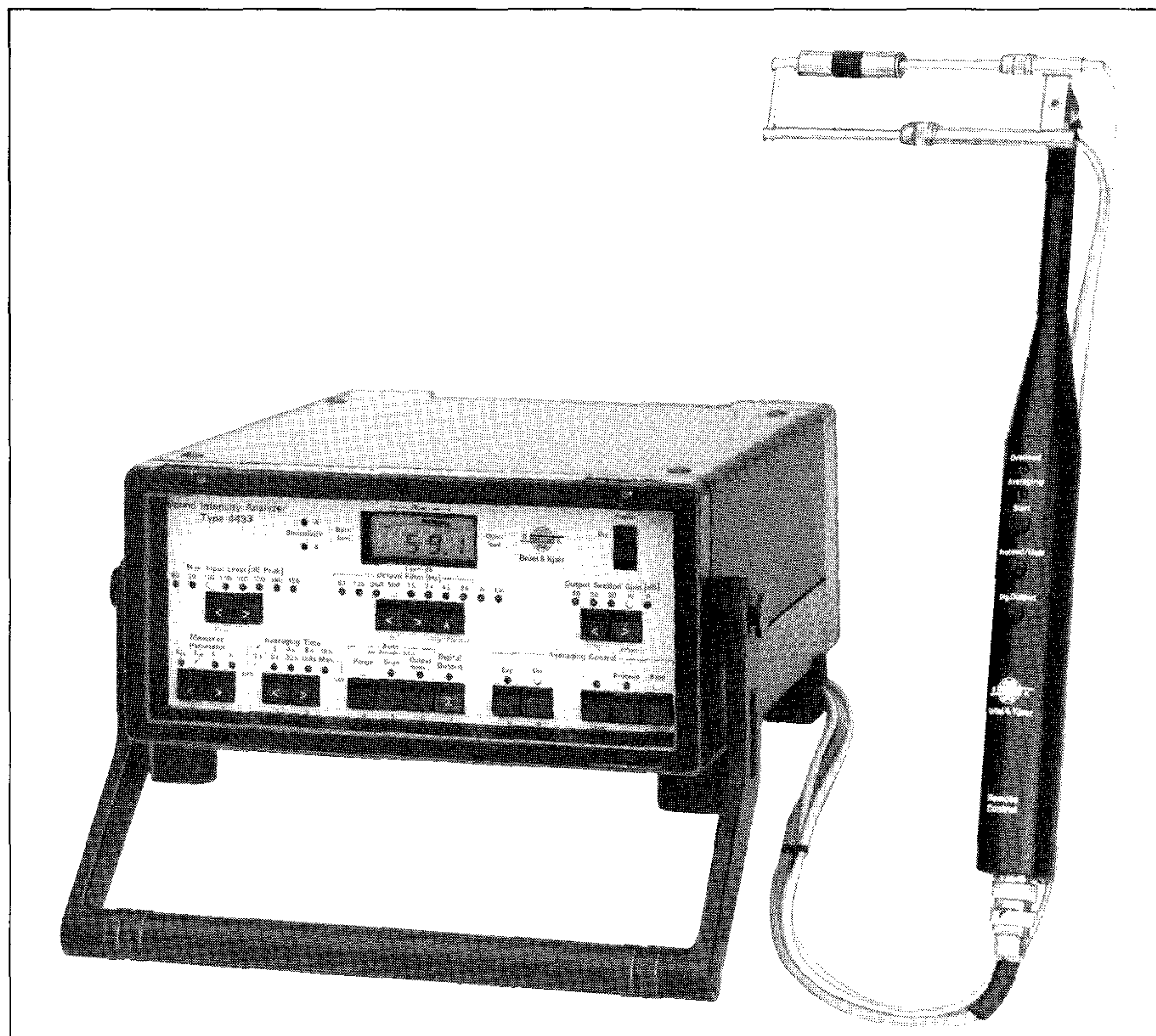
Fig. 4. Sound Intensity Analyzer Type 4433 and Probe Type 3520
