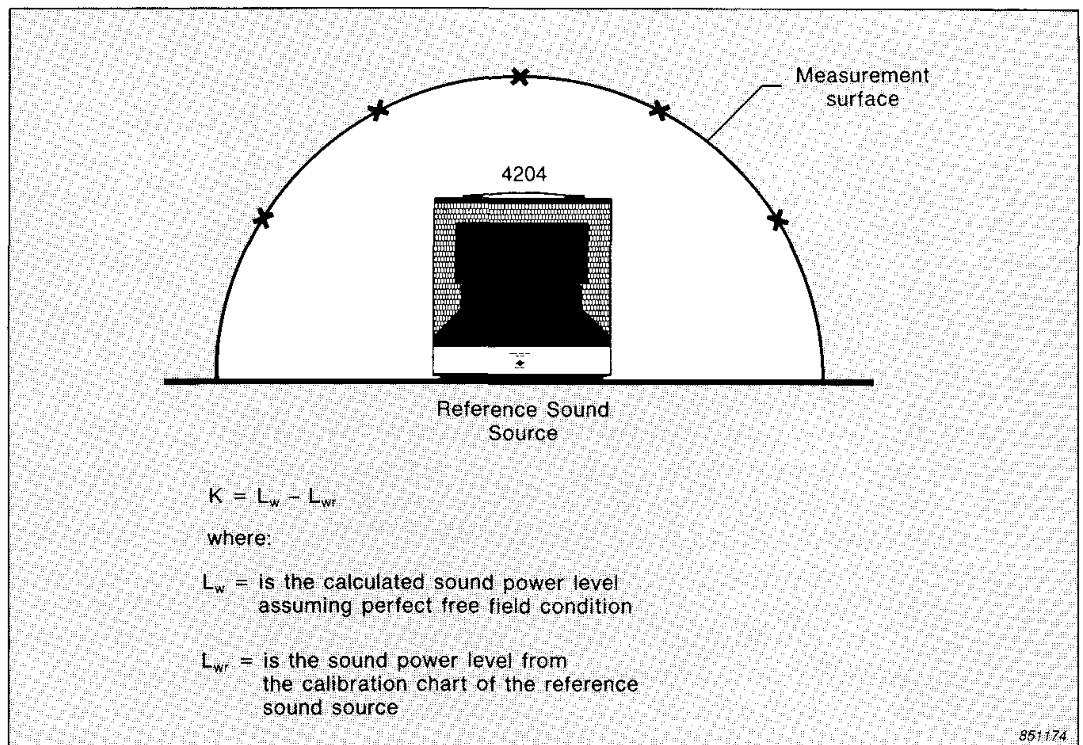
Fig. 9. Measurement of the room correction factor K
