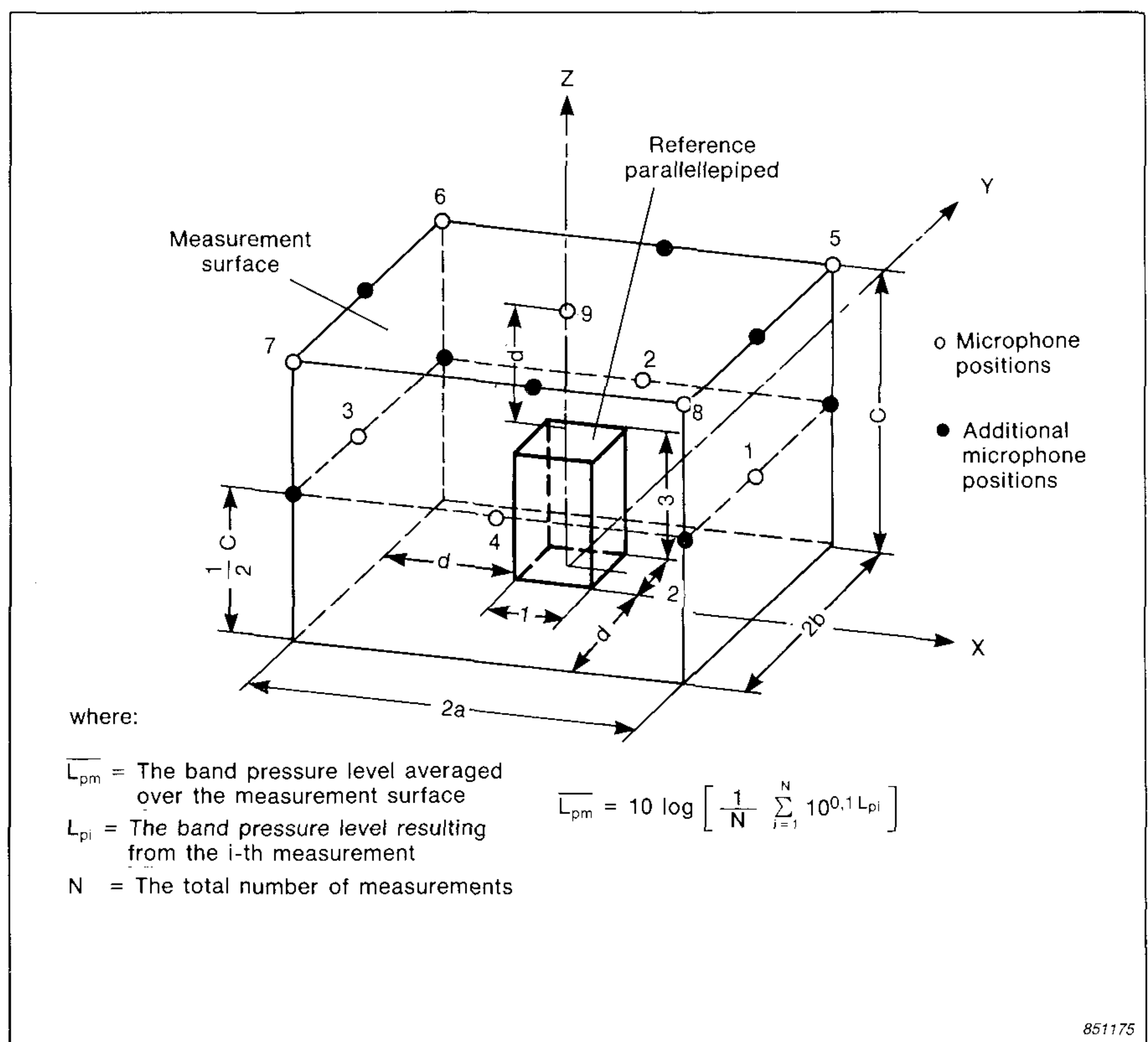
Fig. 6. Parallelepiped surface area according to ISO 3744
