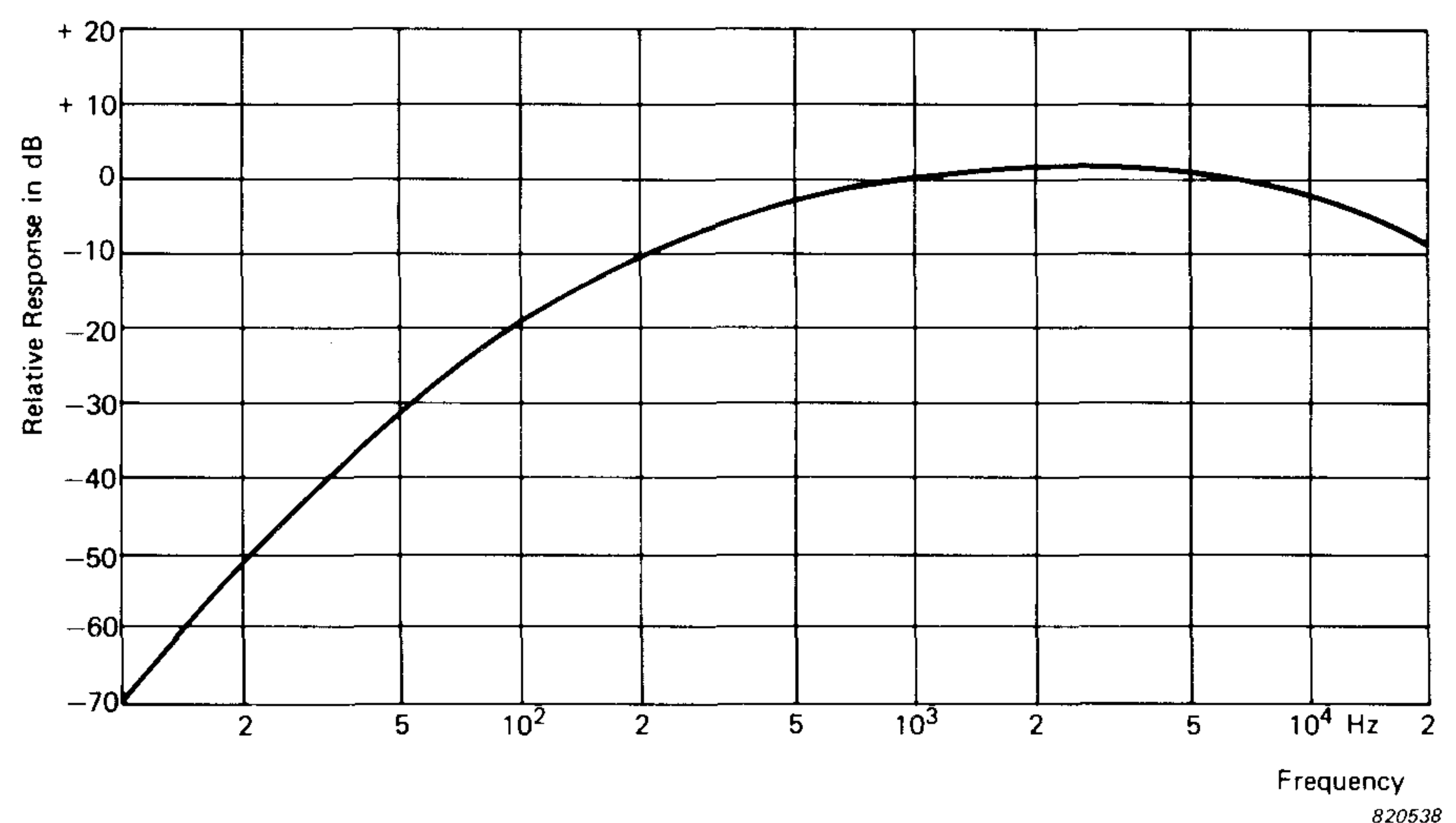
Fig. 3. A-weighting curve
