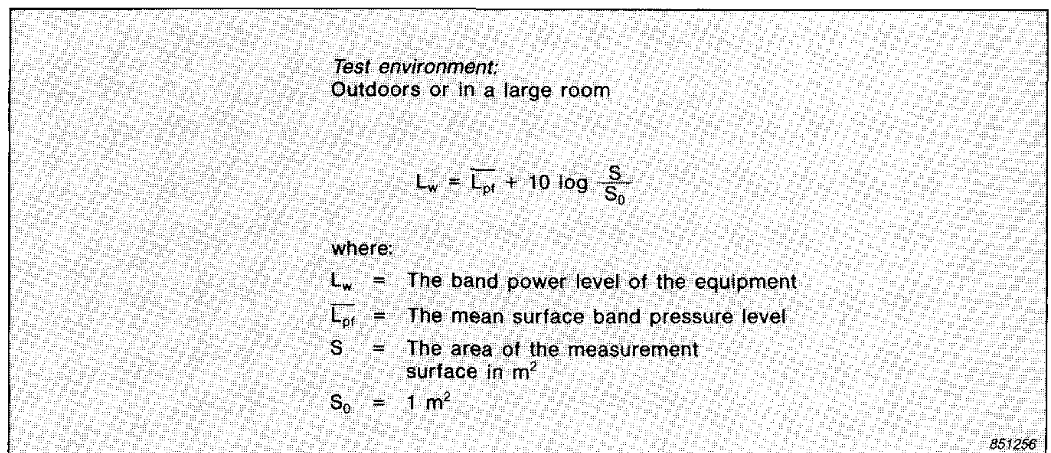
Fig. 10. Calculation of sound power according to ISO 3744
