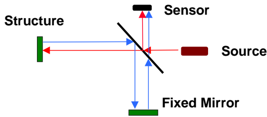
Fig.1 Schematic overview of a Michelson Interferometer. Detector principle is Homodyning. In a practical LDV implementation, "Sensor" would be a photodetector and "Source" would be a laser.
