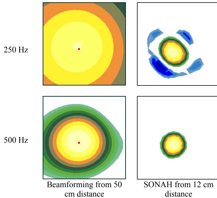
Figure 9: Results from the measurements taken with the set-up in Figure 8. The contour plots all cover a 1m x 1m area and have 10 dB dynamic range. The SONAH plots show Sound Intensity, which can be inwards/negative (blue colors).
