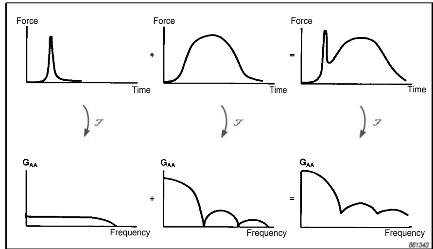
Fig. 4. In practice the impulse applied to a structure is the sum of two separate impulses. The first, parasitic impulse is undesirable, and can to some extent be minimized
