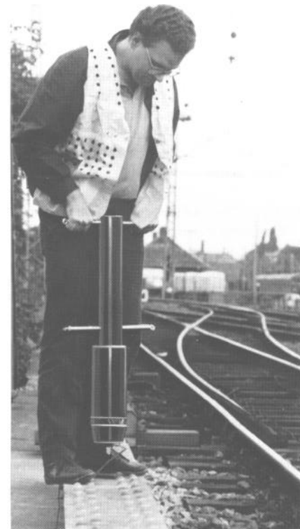
Fig. 6 The operator excited the structure by applying an impact to a small rubber patch placed on the structure
