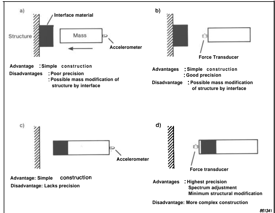
Fig. 2. Four alternative configurations for large impactor design. The configuration in d) gives the optimum performance
