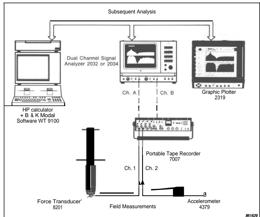
Fig. 5. Field and laboratory instrumentation used for testing a steel girder bridge
