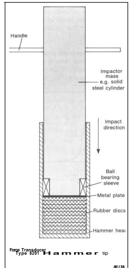
Fig. 3. Assembly drawing of a large impactor using the Brüel & Kjær Force Transducer Type 8201
