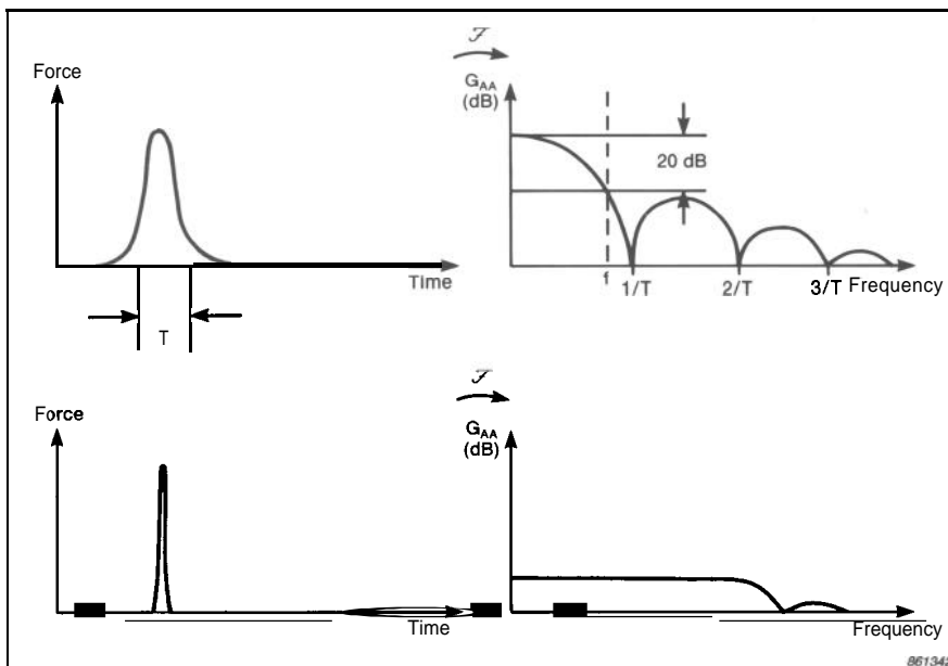
Fig. 1. A broad impulse concentrates the excitation energy at the lower frequencies, whereas a narrow impulse spreads the available energy over a wider frequency range
