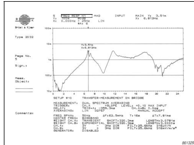
Fig. 8. A typical frequency response function obtained by the test
