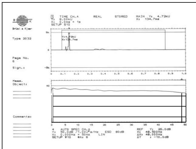
Fig. 7. The Autospectrum verifies that the excitation energy level was adequate within the frequency range of interest
